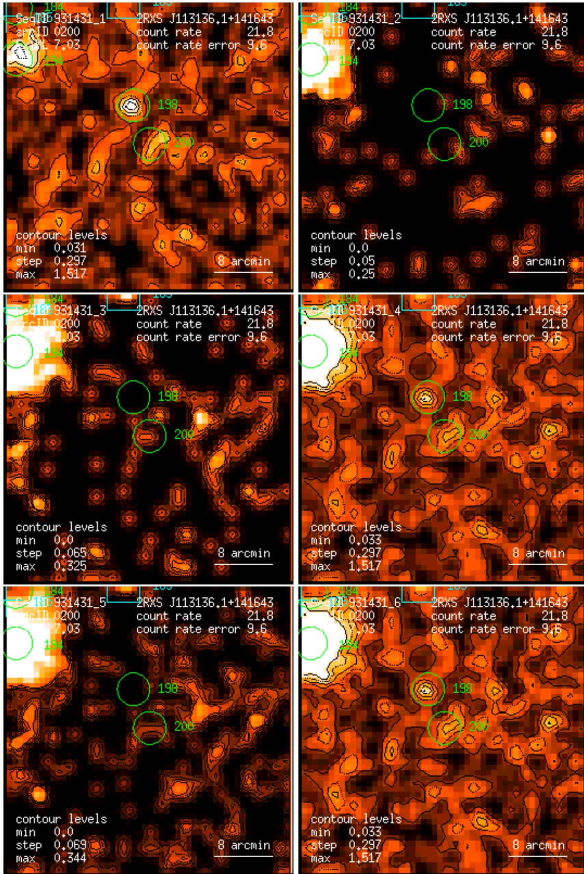
Figure 200: RASS 931431: detection 0200: band rate images, Gaussian filter: (1) PSPC channels 11 – 41, (2) 52 – 90, (3) 91 – 201, (4) 11 – 235, (5) 52 – 201, (6) 11 – 201. Broad band rates in counts/ks. Band rate contour levels in counts/ks/arcmin 2 .
