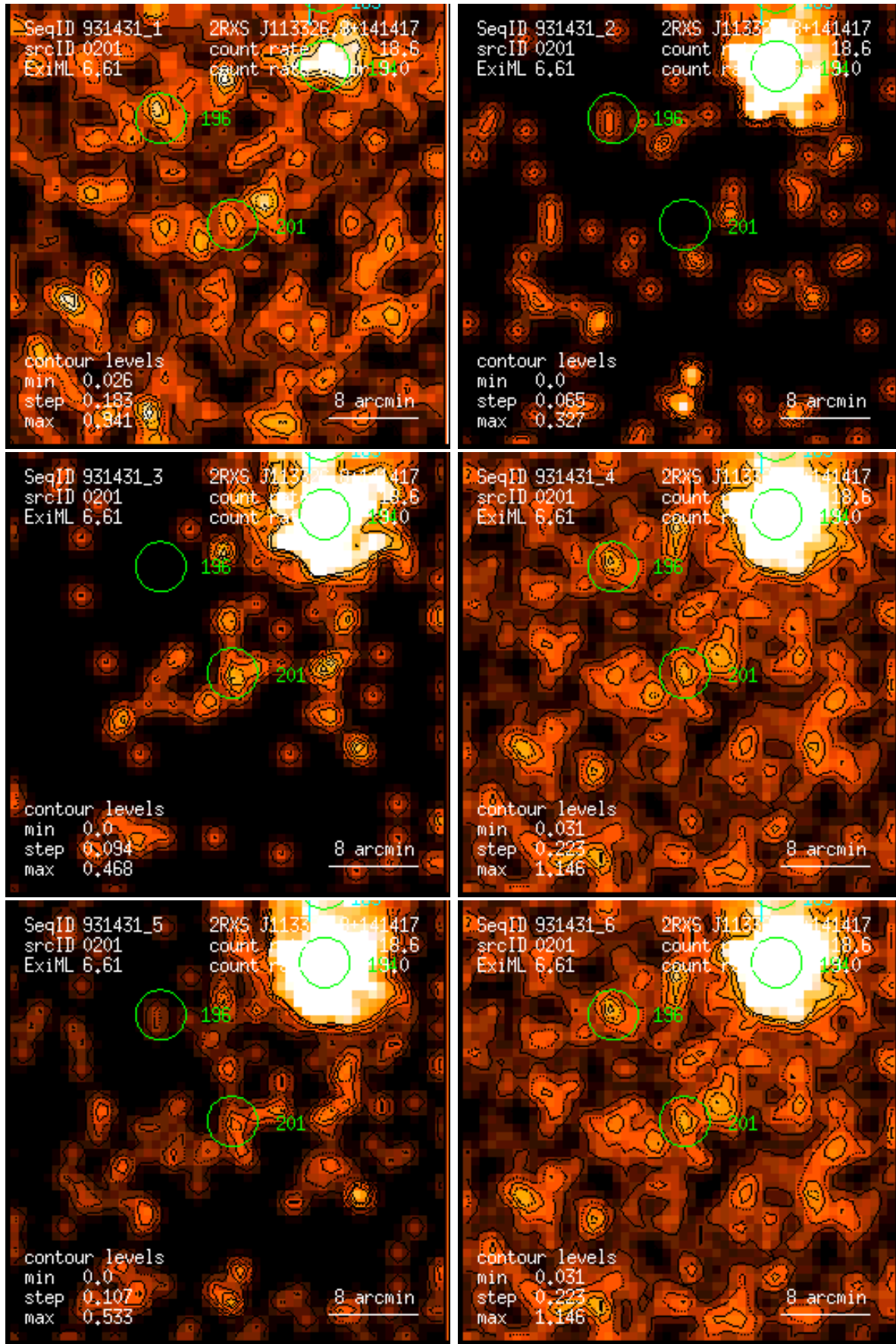
Figure 201: RASS 931431: detection 0201: band rate images, Gaussian filter: (1) PSPC channels 11 – 41, (2) 52 – 90, (3) 91 – 201, (4) 11 – 235, (5) 52 – 201, (6) 11 – 201. Broad band rates in counts/ks. Band rate contour levels in counts/ks/arcmin 2 .
