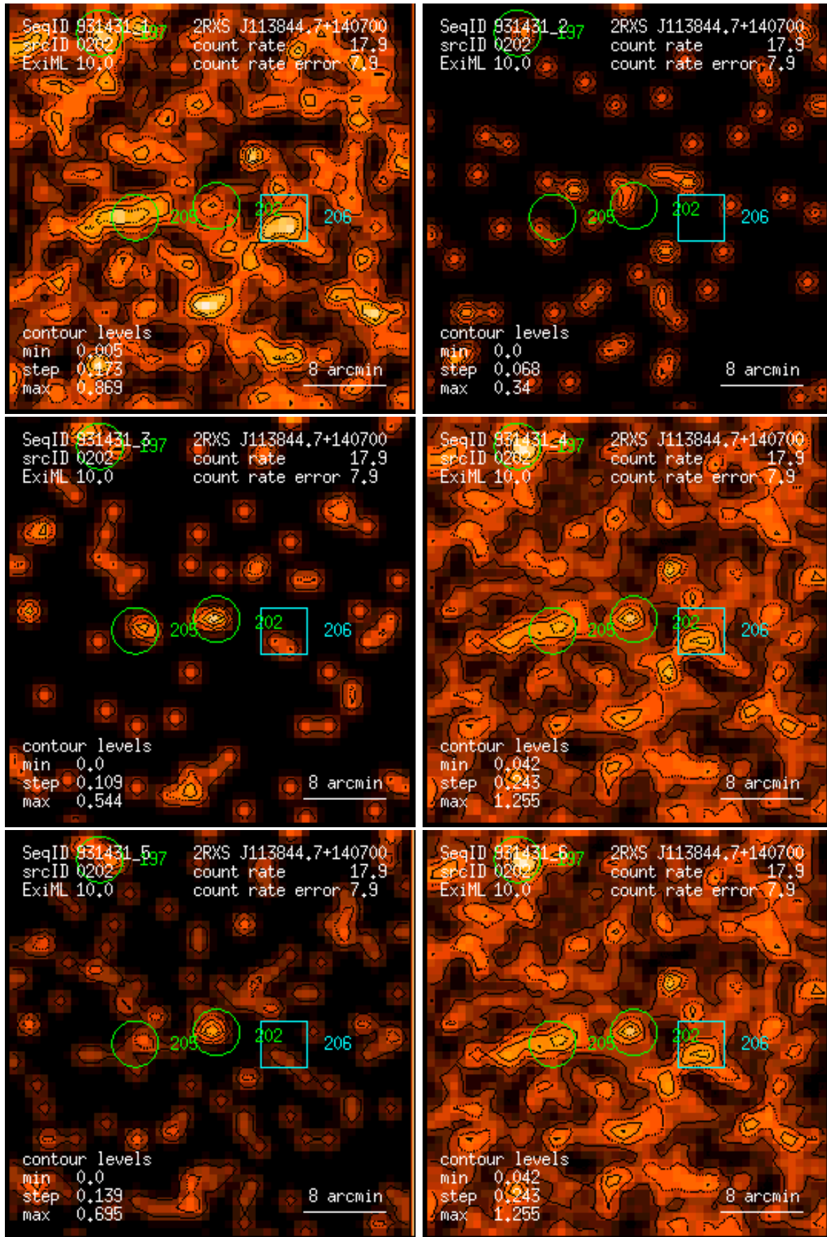
Figure 202: RASS 931431: detection 0202: band rate images, Gaussian filter: (1) PSPC channels 11 – 41, (2) 52 – 90, (3) 91 – 201, (4) 11 – 235, (5) 52 – 201, (6) 11 – 201. Broad band rates in counts/ks. Band rate contour levels in counts/ks/arcmin 2 .
