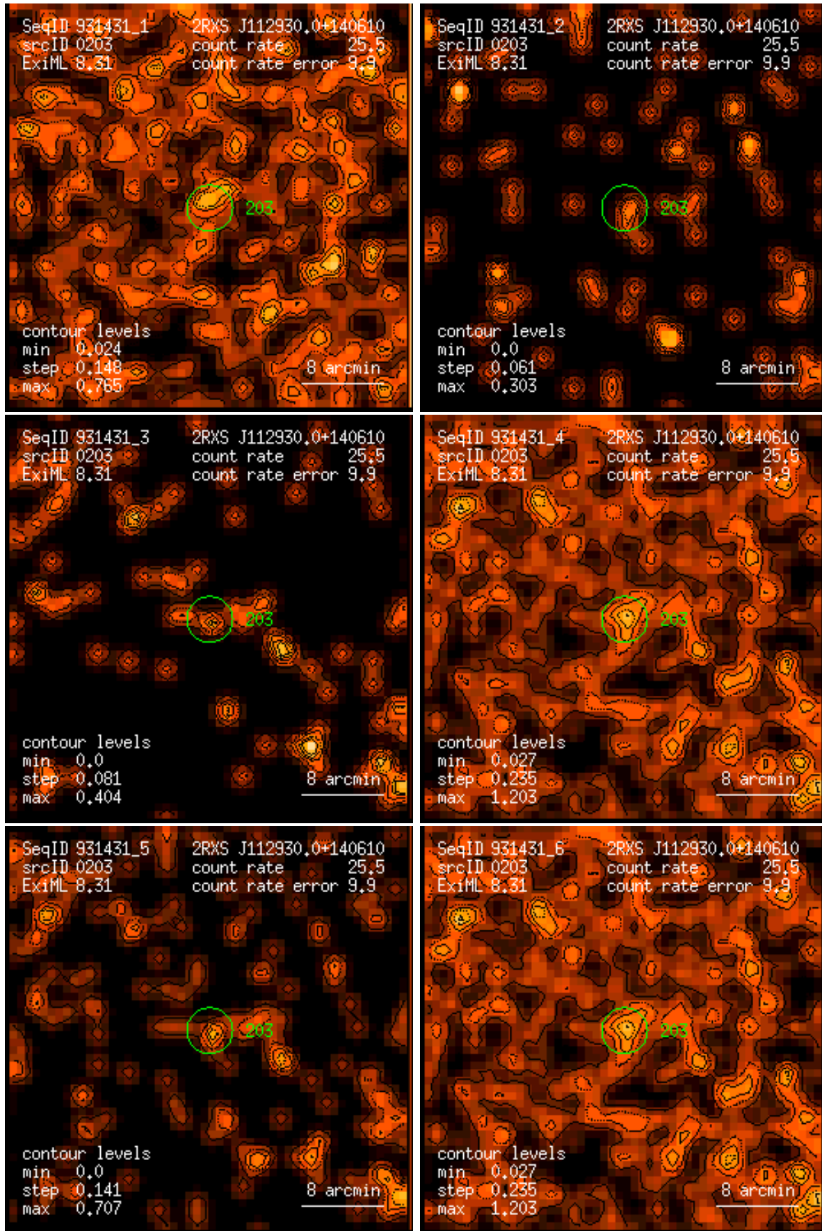
Figure 203: RASS 931431: detection 0203: band rate images, Gaussian filter: (1) PSPC channels 11 – 41, (2) 52 – 90, (3) 91 – 201, (4) 11 – 235, (5) 52 – 201, (6) 11 – 201. Broad band rates in counts/ks. Band rate contour levels in counts/ks/arcmin 2 .
