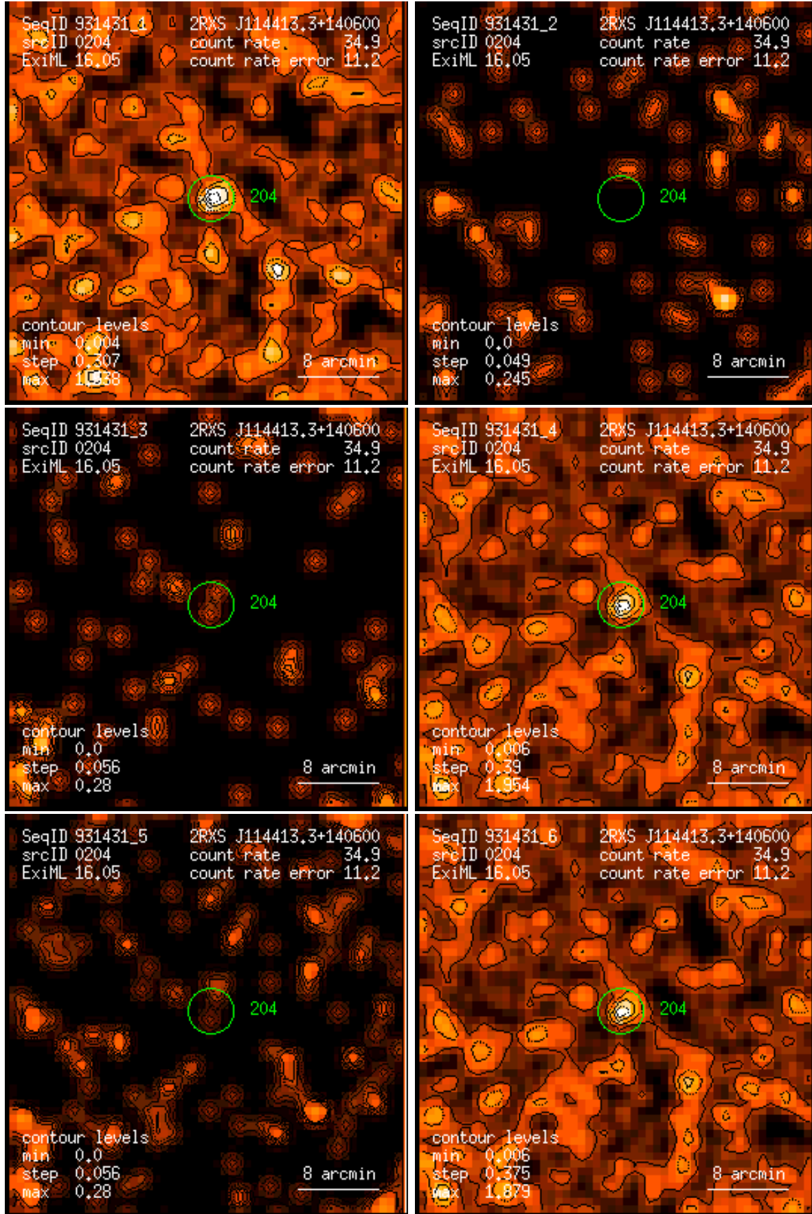
Figure 204: RASS 931431: detection 0204: band rate images, Gaussian filter: (1) PSPC channels 11 – 41, (2) 52 – 90, (3) 91 – 201, (4) 11 – 235, (5) 52 – 201, (6) 11 – 201. Broad band rates in counts/ks. Band rate contour levels in counts/ks/arcmin 2 .
