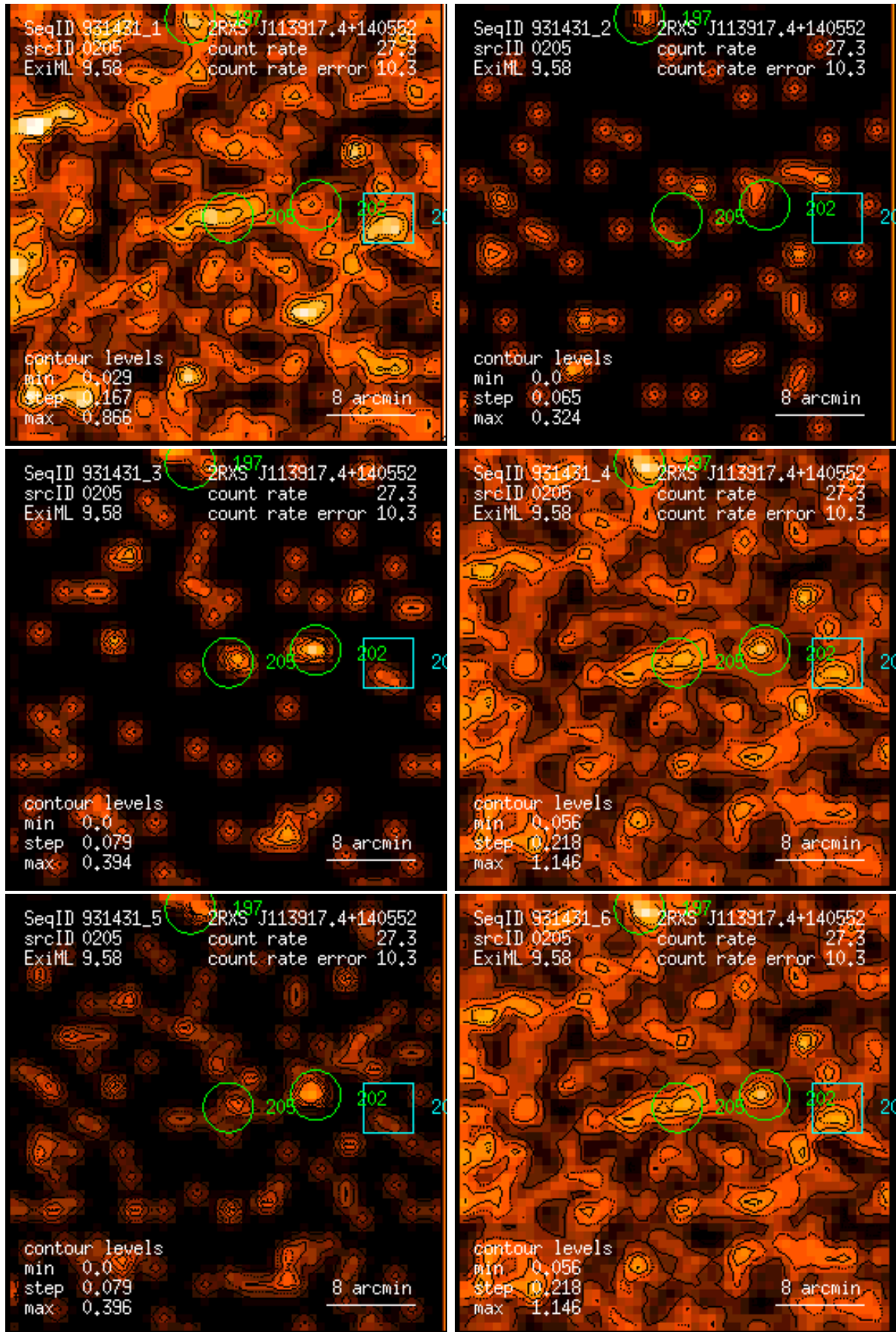
Figure 205: RASS 931431: detection 0205: band rate images, Gaussian filter: (1) PSPC channels 11 – 41, (2) 52 – 90, (3) 91 – 201, (4) 11 – 235, (5) 52 – 201, (6) 11 – 201. Broad band rates in counts/ks. Band rate contour levels in counts/ks/arcmin 2 .
