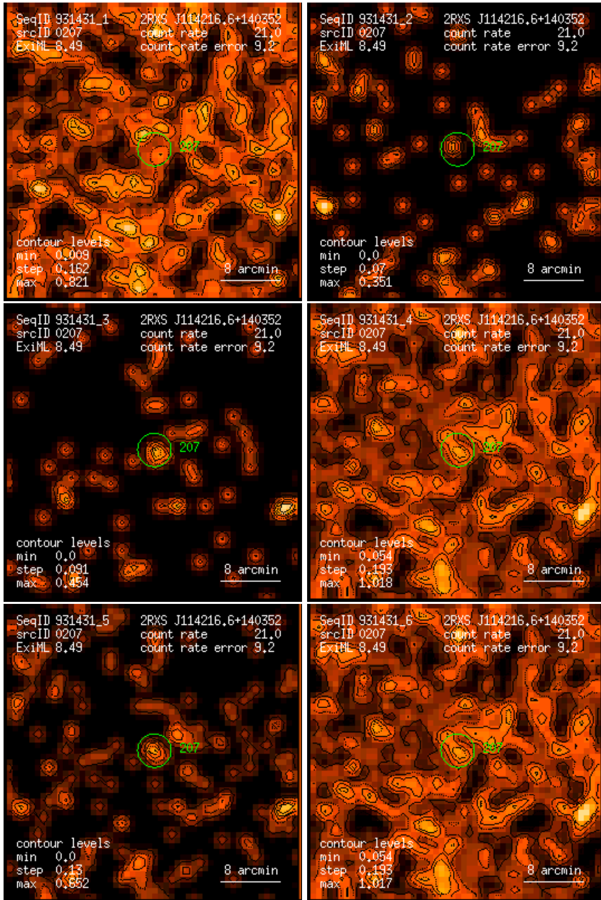
Figure 207: RASS 931431: detection 0207: band rate images, Gaussian filter: (1) PSPC channels 11 – 41, (2) 52 – 90, (3) 91 – 201, (4) 11 – 235, (5) 52 – 201, (6) 11 – 201. Broad band rates in counts/ks. Band rate contour levels in counts/ks/arcmin 2 .
