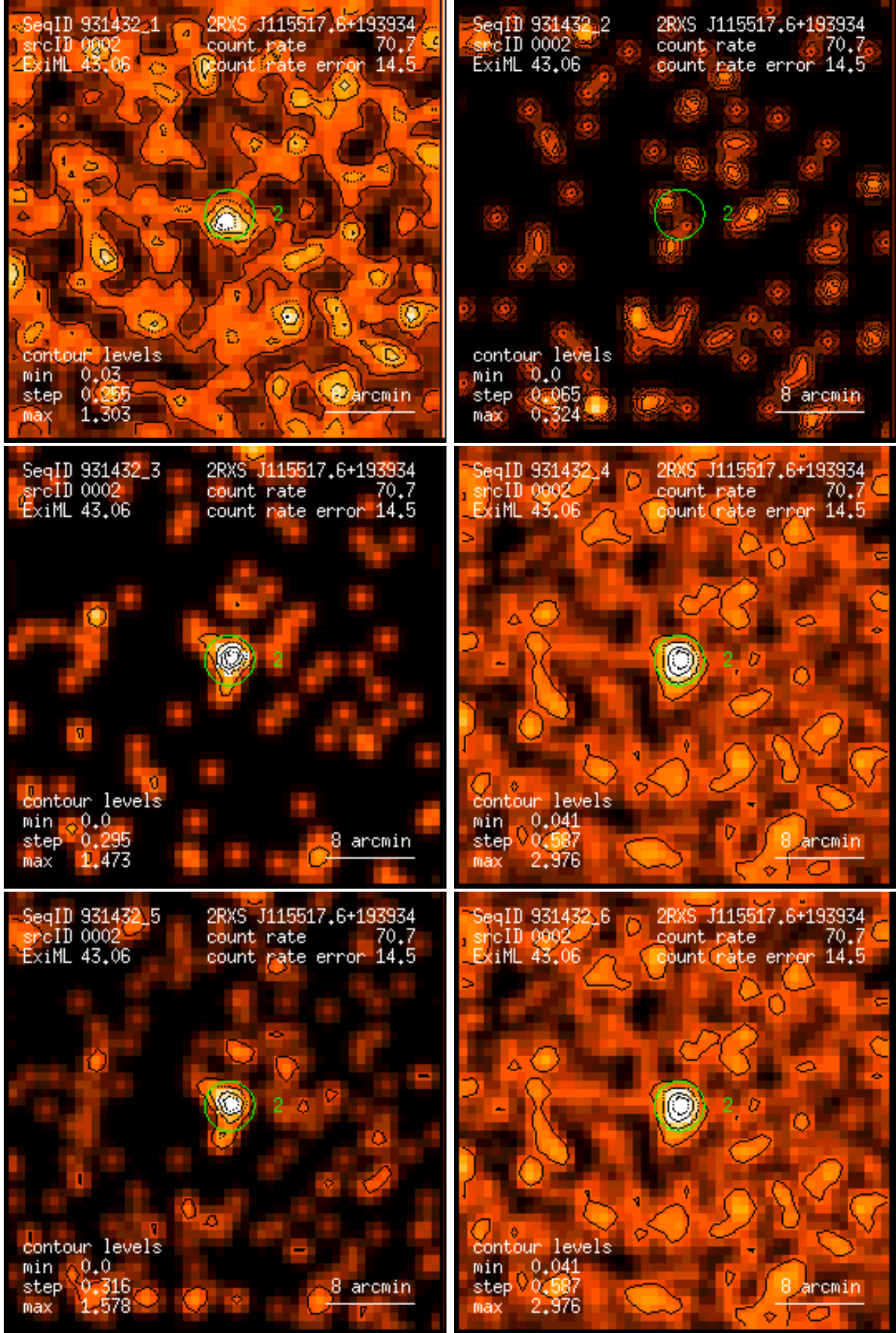
Figure 2: RASS 931432: detection 0002: band rate images, Gaussian filter: (1) PSPC channels 11 – 41, (2) 52 – 90, (3) 91 – 201, (4) 11 – 235, (5) 52 – 201, (6) 11 – 201. Broad band rates in counts/ks. Band rate contour levels in counts/ks/arcmin 2 .
