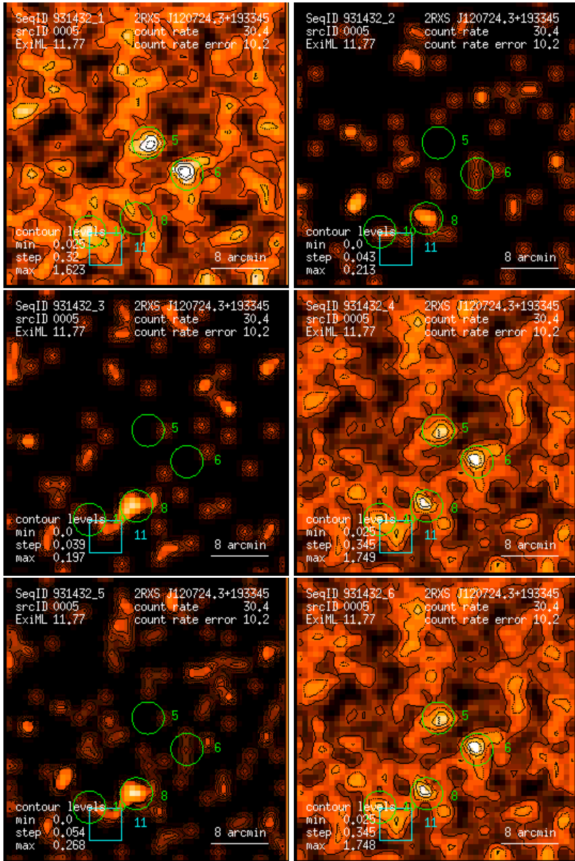
Figure 5: RASS 931432: detection 0005: band rate images, Gaussian filter: (1) PSPC channels 11 – 41, (2) 52 – 90, (3) 91 – 201, (4) 11 – 235, (5) 52 – 201, (6) 11 – 201. Broad band rates in counts/ks. Band rate contour levels in counts/ks/arcmin 2 .
