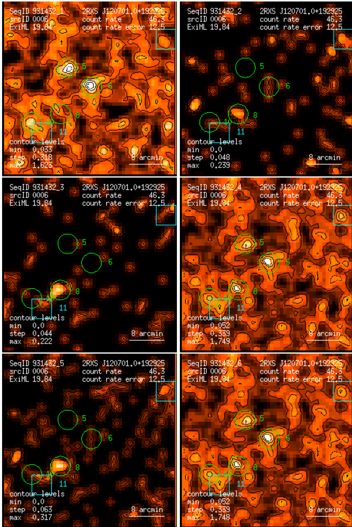
Figure 6: RASS 931432: detection 0006: band rate images, Gaussian filter: (1) PSPC channels 11 – 41, (2) 52 – 90, (3) 91 – 201, (4) 11 – 235, (5) 52 – 201, (6) 11 – 201. Broad band rates in counts/ks. Band rate contour levels in counts/ks/arcmin 2 .
