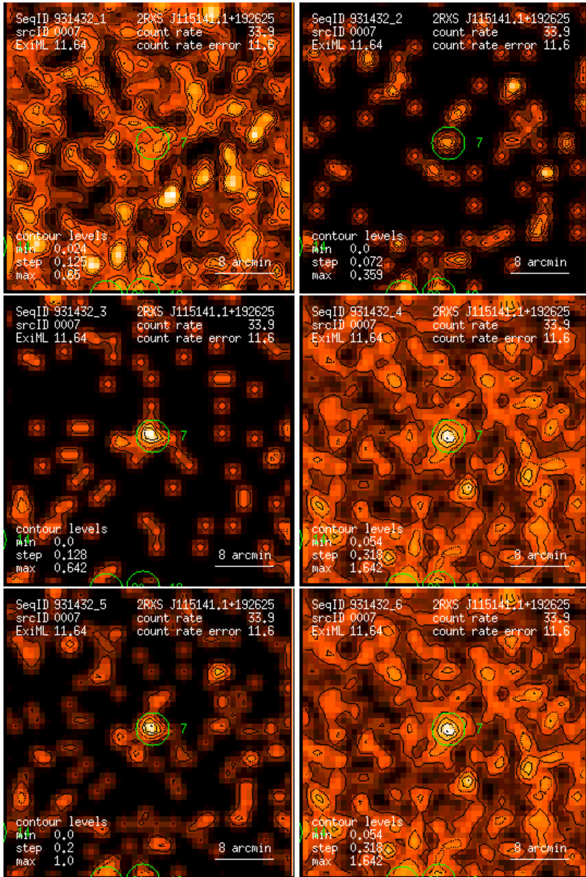
Figure 7: RASS 931432: detection 0007: band rate images, Gaussian filter: (1) PSPC channels 11 – 41, (2) 52 – 90, (3) 91 – 201, (4) 11 – 235, (5) 52 – 201, (6) 11 – 201. Broad band rates in counts/ks. Band rate contour levels in counts/ks/arcmin 2 .
