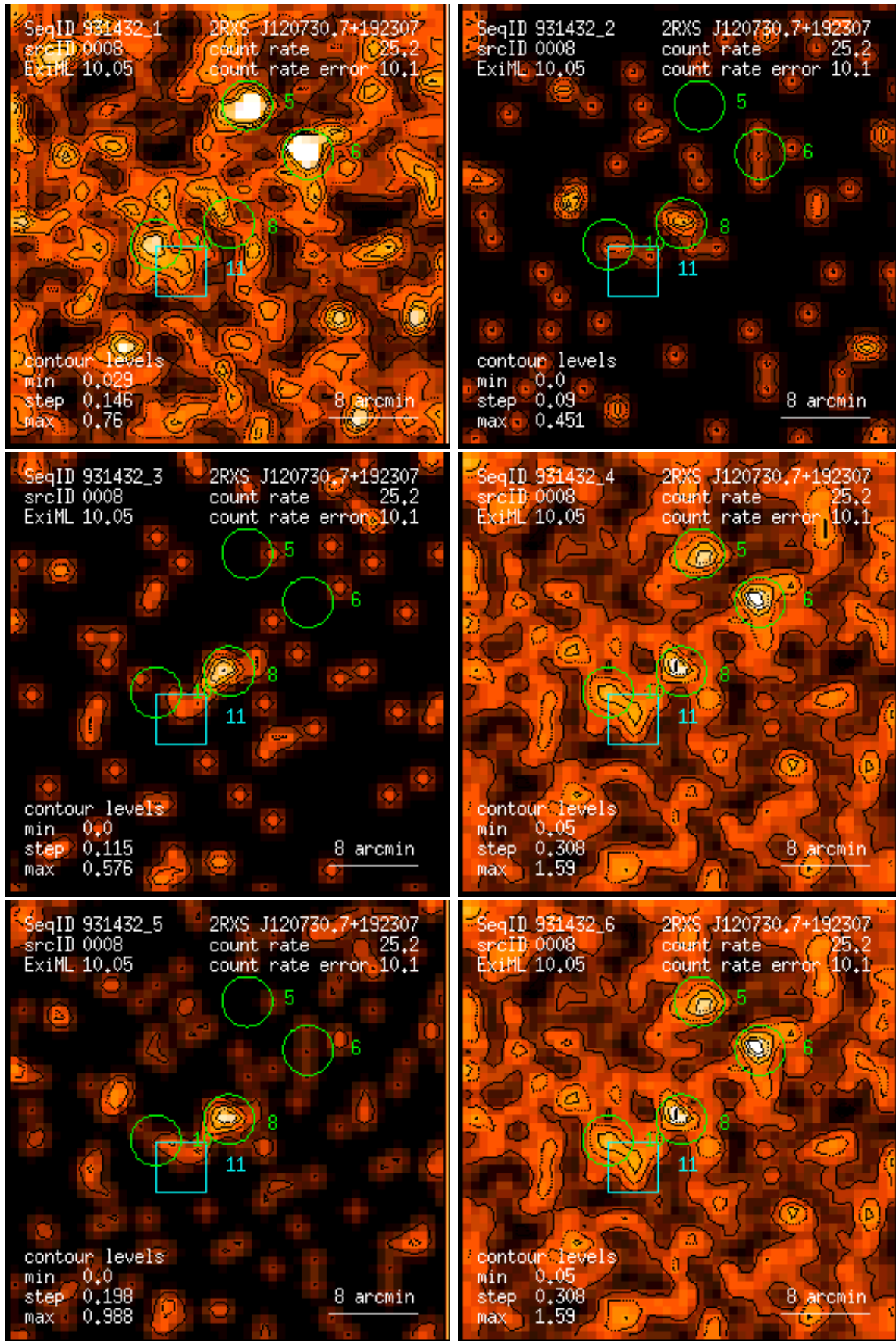
Figure 8: RASS 931432: detection 0008: band rate images, Gaussian filter: (1) PSPC channels 11 – 41, (2) 52 – 90, (3) 91 – 201, (4) 11 – 235, (5) 52 – 201, (6) 11 – 201. Broad band rates in counts/ks. Band rate contour levels in counts/ks/arcmin 2 .
