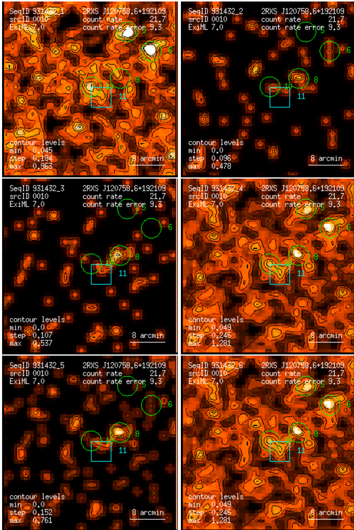
Figure 10: RASS 931432: detection 0010: band rate images, Gaussian filter: (1) PSPC channels 11 – 41, (2) 52 – 90, (3) 91 – 201, (4) 11 – 235, (5) 52 – 201, (6) 11 – 201. Broad band rates in counts/ks. Band rate contour levels in counts/ks/arcmin 2 .
