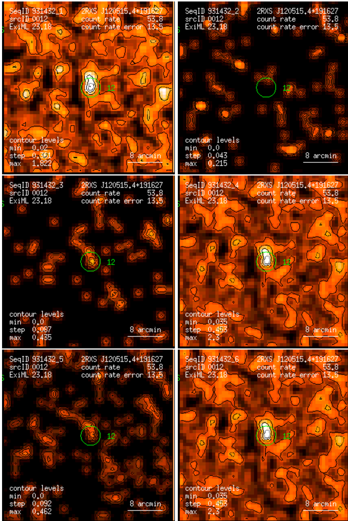
Figure 12: RASS 931432: detection 0012: band rate images, Gaussian filter: (1) PSPC channels 11 – 41, (2) 52 – 90, (3) 91 – 201, (4) 11 – 235, (5) 52 – 201, (6) 11 – 201. Broad band rates in counts/ks. Band rate contour levels in counts/ks/arcmin 2 .
