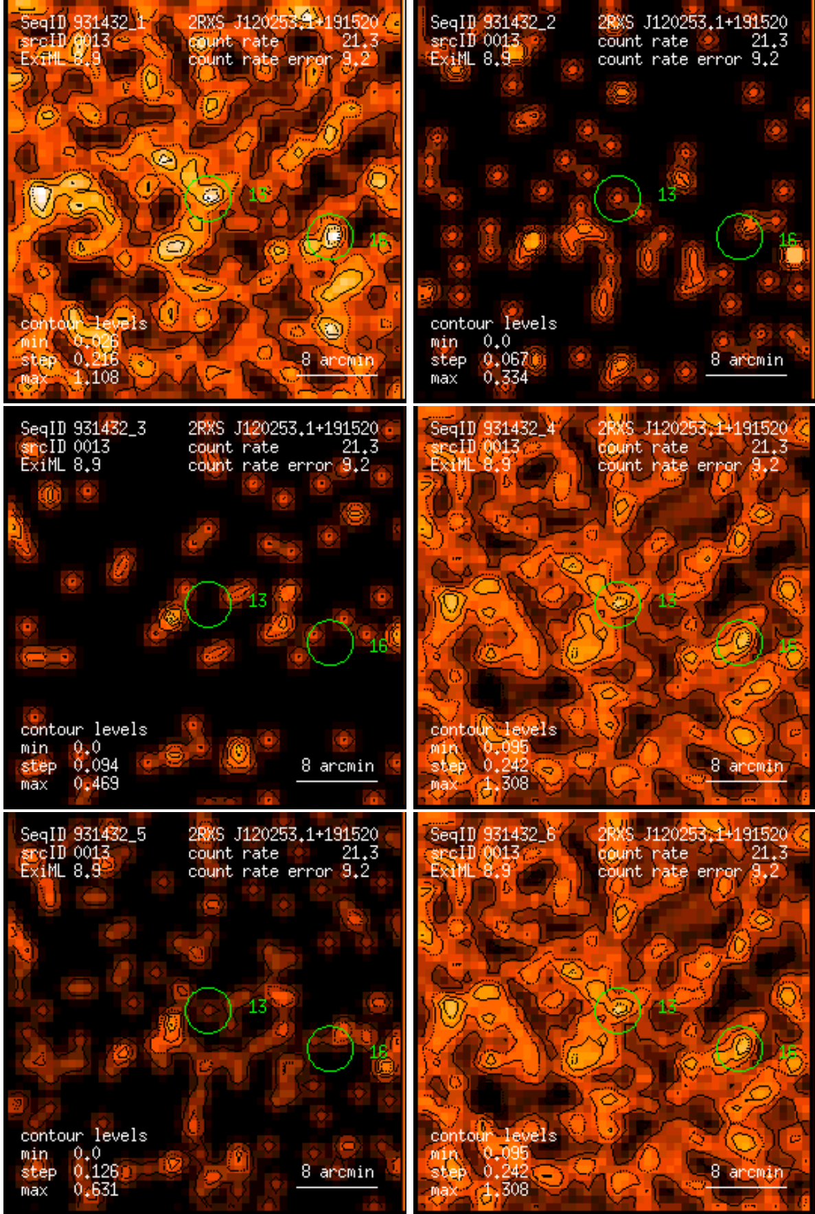
Figure 13: RASS 931432: detection 0013: band rate images, Gaussian filter: (1) PSPC channels 11 – 41, (2) 52 – 90, (3) 91 – 201, (4) 11 – 235, (5) 52 – 201, (6) 11 – 201. Broad band rates in counts/ks. Band rate contour levels in counts/ks/arcmin 2 .
