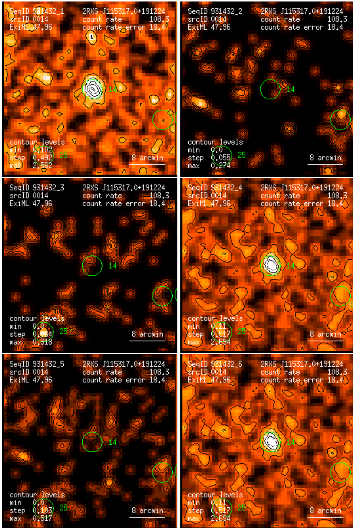
Figure 14: RASS 931432: detection 0014: band rate images, Gaussian filter: (1) PSPC channels 11 – 41, (2) 52 – 90, (3) 91 – 201, (4) 11 – 235, (5) 52 – 201, (6) 11 – 201. Broad band rates in counts/ks. Band rate contour levels in counts/ks/arcmin 2 .
