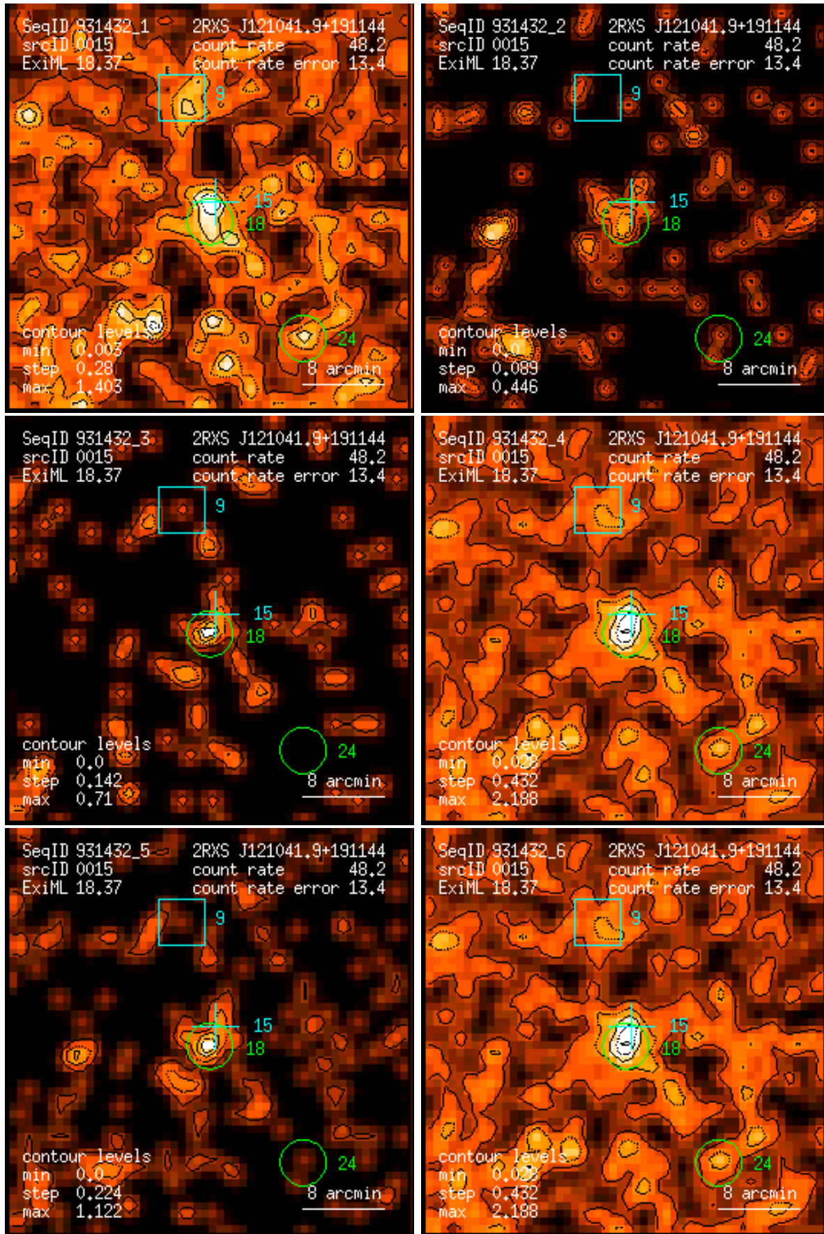
Figure 15: RASS 931432: detection 0015: band rate images, Gaussian filter: (1) PSPC channels 11 – 41, (2) 52 – 90, (3) 91 – 201, (4) 11 – 235, (5) 52 – 201, (6) 11 – 201. Broad band rates in counts/ks. Band rate contour levels in counts/ks/arcmin 2 .
