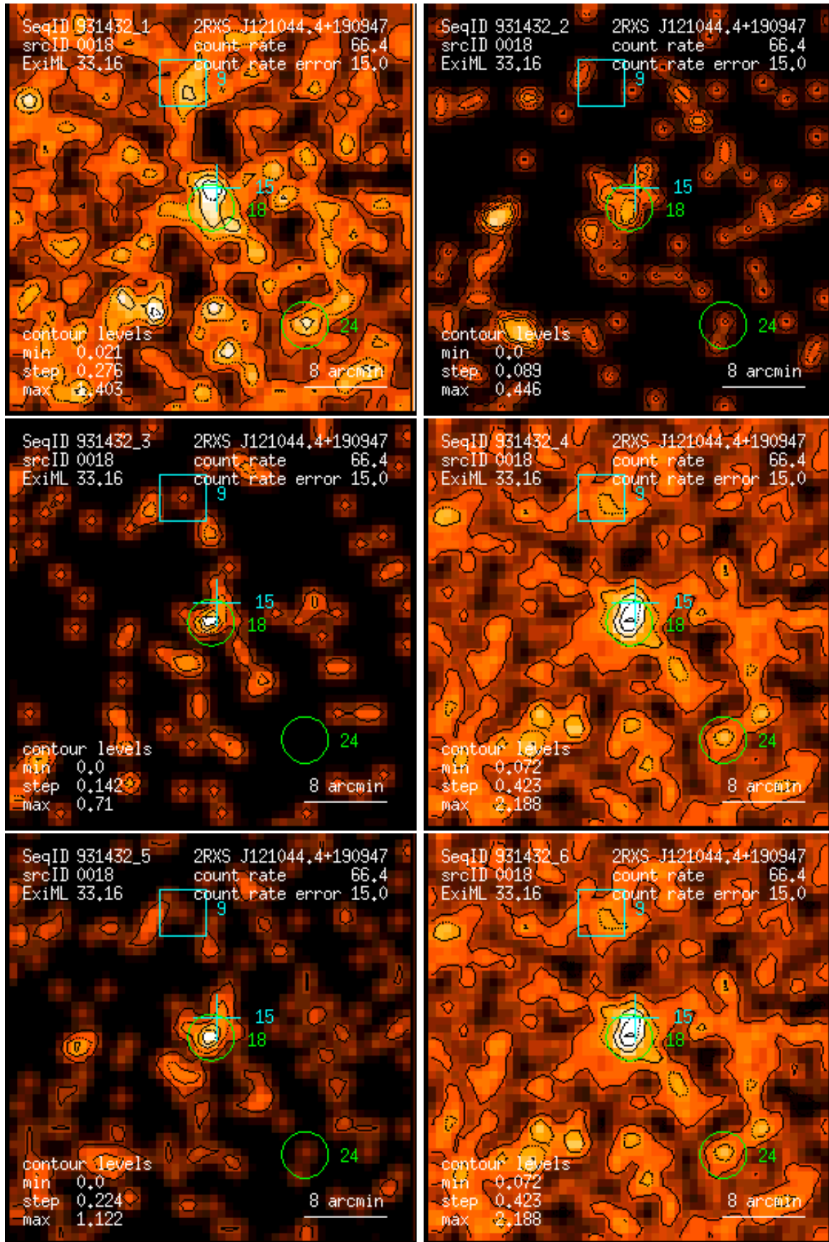
Figure 18: RASS 931432: detection 0018: band rate images, Gaussian filter: (1) PSPC channels 11 – 41, (2) 52 – 90, (3) 91 – 201, (4) 11 – 235, (5) 52 – 201, (6) 11 – 201. Broad band rates in counts/ks. Band rate contour levels in counts/ks/arcmin 2 .
