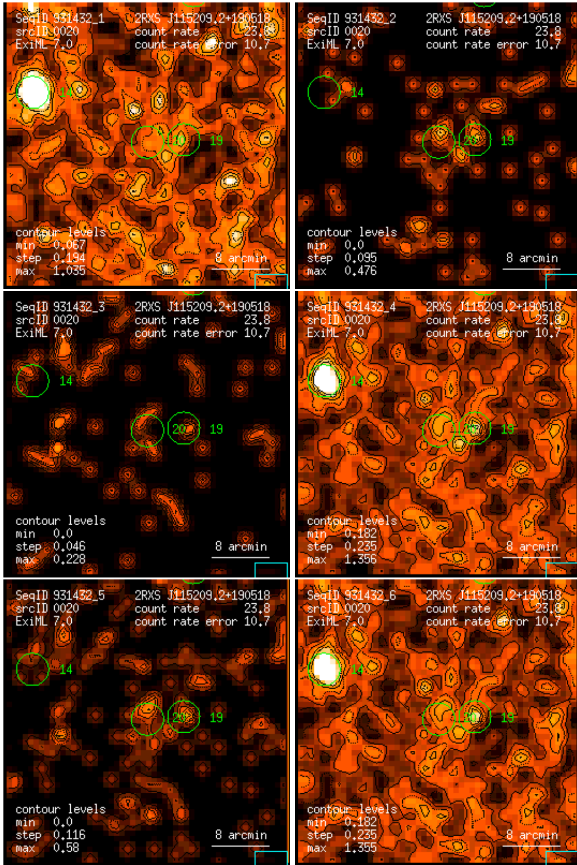
Figure 20: RASS 931432: detection 0020: band rate images, Gaussian filter: (1) PSPC channels 11 – 41, (2) 52 – 90, (3) 91 – 201, (4) 11 – 235, (5) 52 – 201, (6) 11 – 201. Broad band rates in counts/ks. Band rate contour levels in counts/ks/arcmin 2 .
