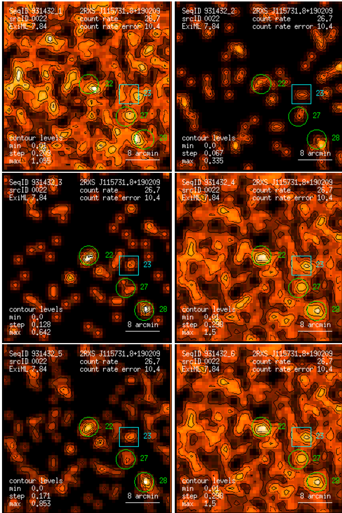
Figure 22: RASS 931432: detection 0022: band rate images, Gaussian filter: (1) PSPC channels 11 – 41, (2) 52 – 90, (3) 91 – 201, (4) 11 – 235, (5) 52 – 201, (6) 11 – 201. Broad band rates in counts/ks. Band rate contour levels in counts/ks/arcmin 2 .
