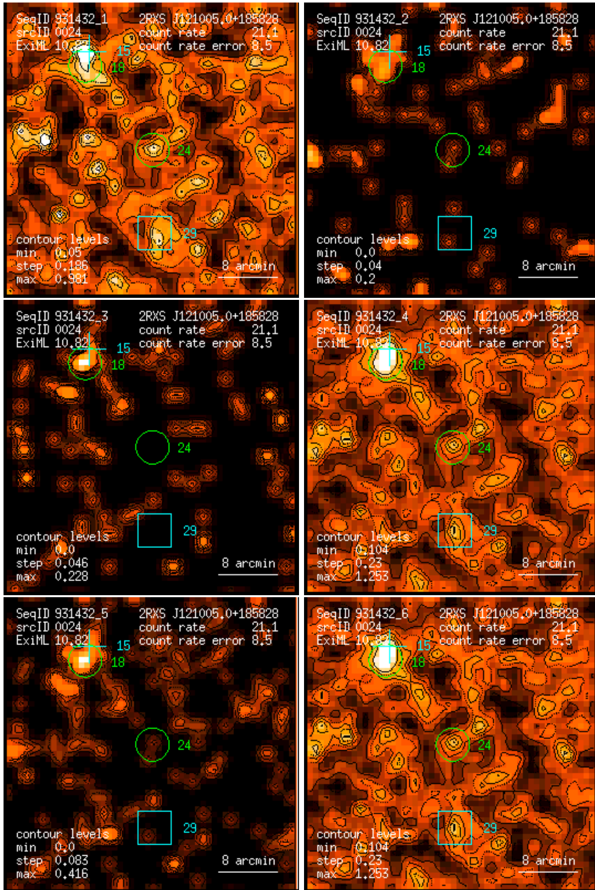
Figure 24: RASS 931432: detection 0024: band rate images, Gaussian filter: (1) PSPC channels 11 – 41, (2) 52 – 90, (3) 91 – 201, (4) 11 – 235, (5) 52 – 201, (6) 11 – 201. Broad band rates in counts/ks. Band rate contour levels in counts/ks/arcmin 2 .
