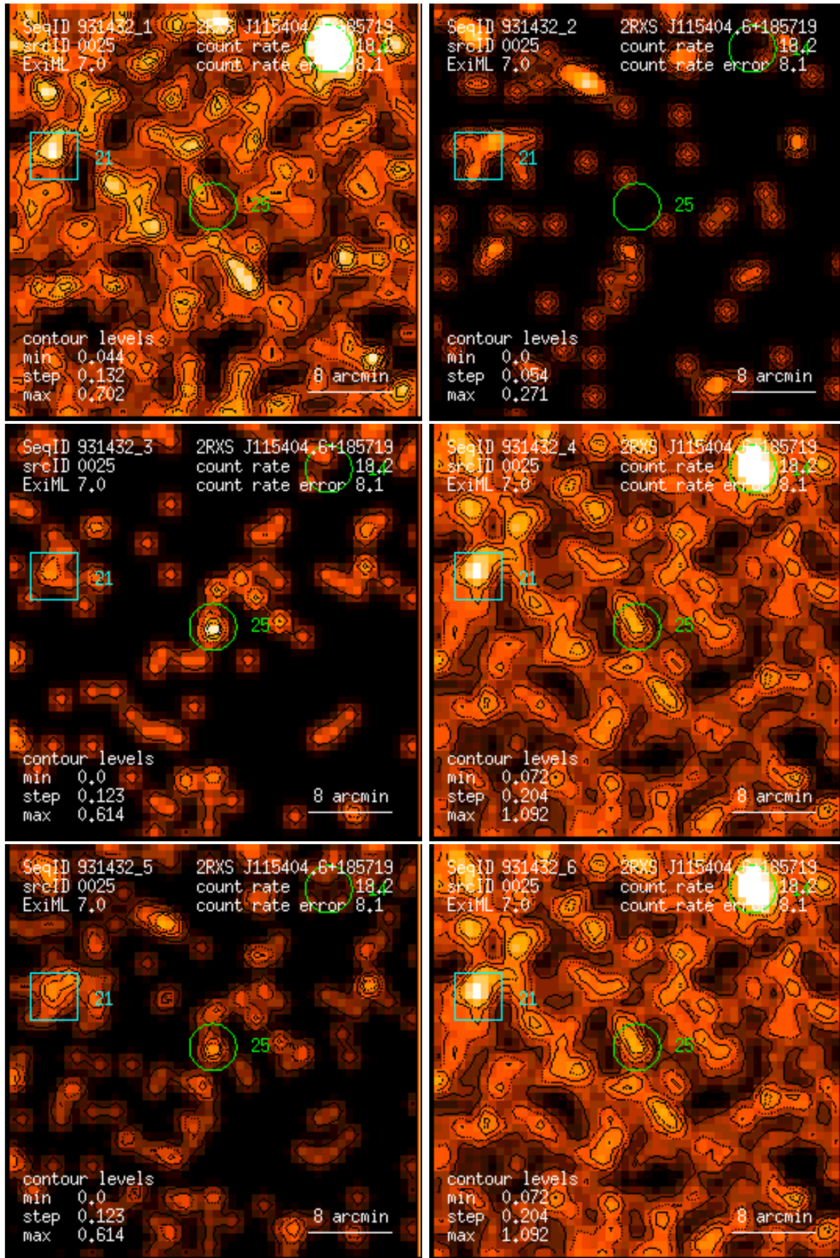
Figure 25: RASS 931432: detection 0025: band rate images, Gaussian filter: (1) PSPC channels 11 – 41, (2) 52 – 90, (3) 91 – 201, (4) 11 – 235, (5) 52 – 201, (6) 11 – 201. Broad band rates in counts/ks. Band rate contour levels in counts/ks/arcmin 2 .
