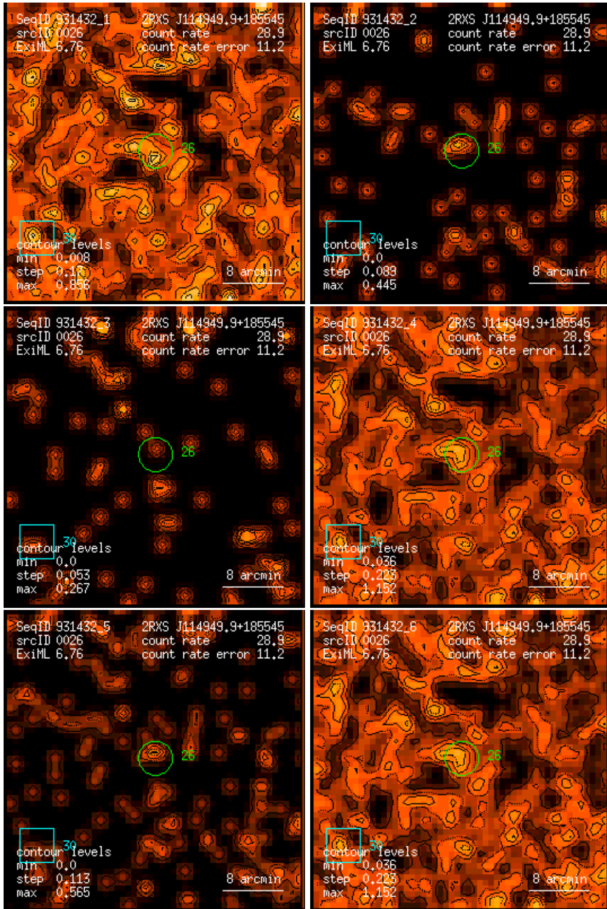
Figure 26: RASS 931432: detection 0026: band rate images, Gaussian filter: (1) PSPC channels 11 – 41, (2) 52 – 90, (3) 91 – 201, (4) 11 – 235, (5) 52 – 201, (6) 11 – 201. Broad band rates in counts/ks. Band rate contour levels in counts/ks/arcmin 2 .
