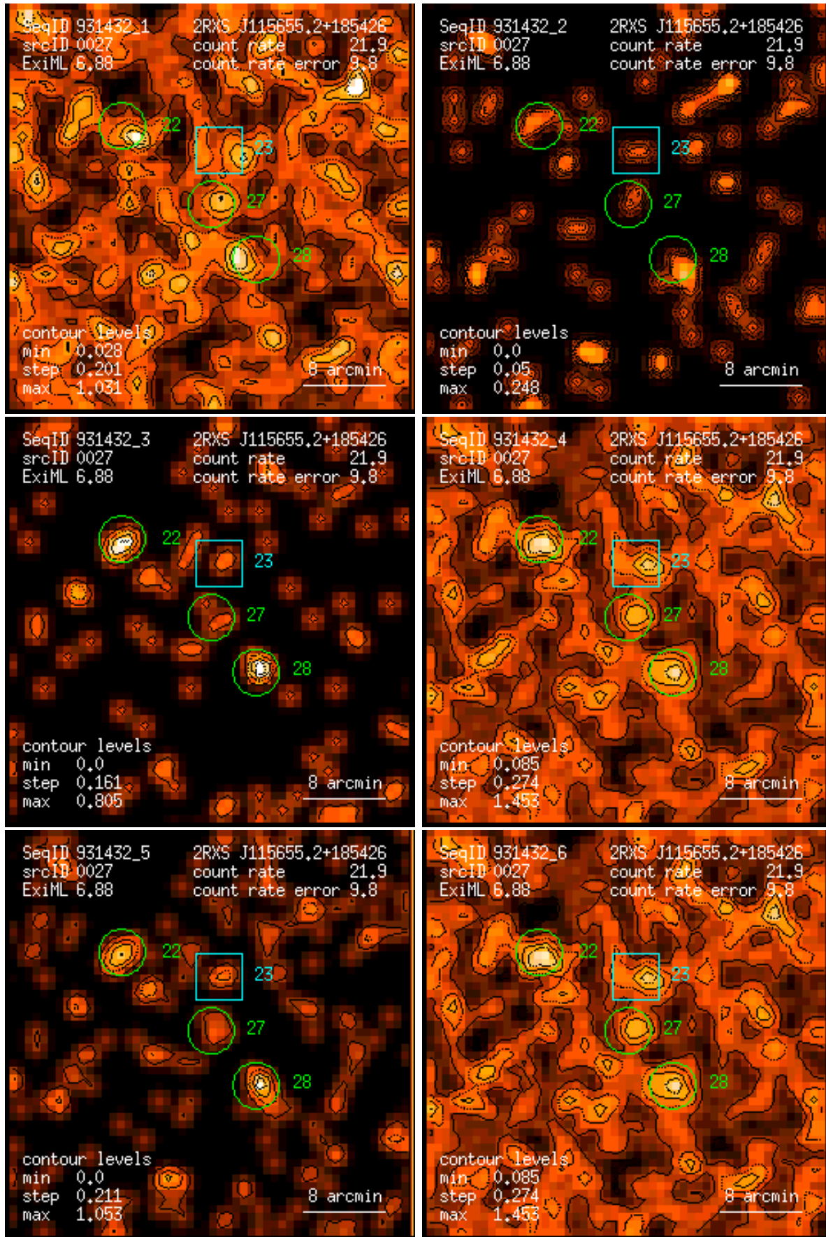
Figure 27: RASS 931432: detection 0027: band rate images, Gaussian filter: (1) PSPC channels 11 – 41, (2) 52 – 90, (3) 91 – 201, (4) 11 – 235, (5) 52 – 201, (6) 11 – 201. Broad band rates in counts/ks. Band rate contour levels in counts/ks/arcmin 2 .
