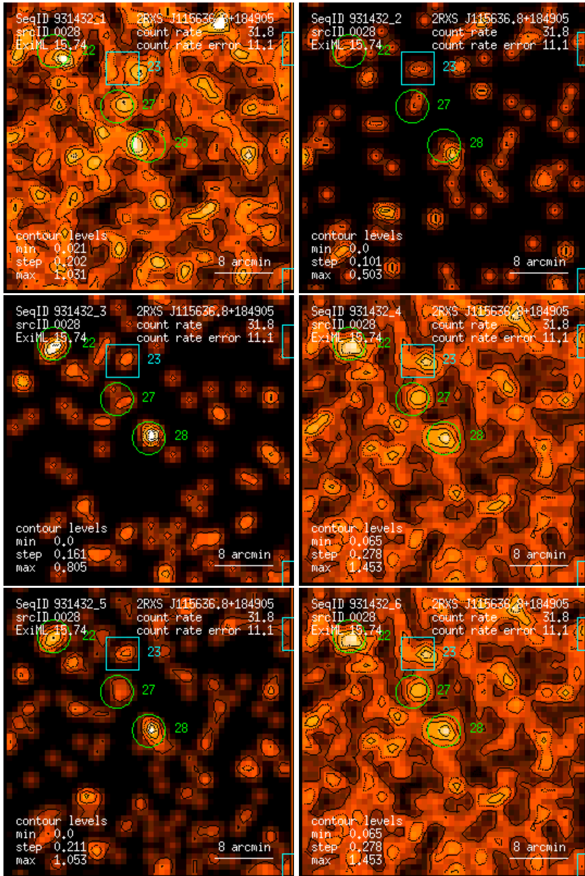
Figure 28: RASS 931432: detection 0028: band rate images, Gaussian filter: (1) PSPC channels 11 – 41, (2) 52 – 90, (3) 91 – 201, (4) 11 – 235, (5) 52 – 201, (6) 11 – 201. Broad band rates in counts/ks. Band rate contour levels in counts/ks/arcmin 2 .
