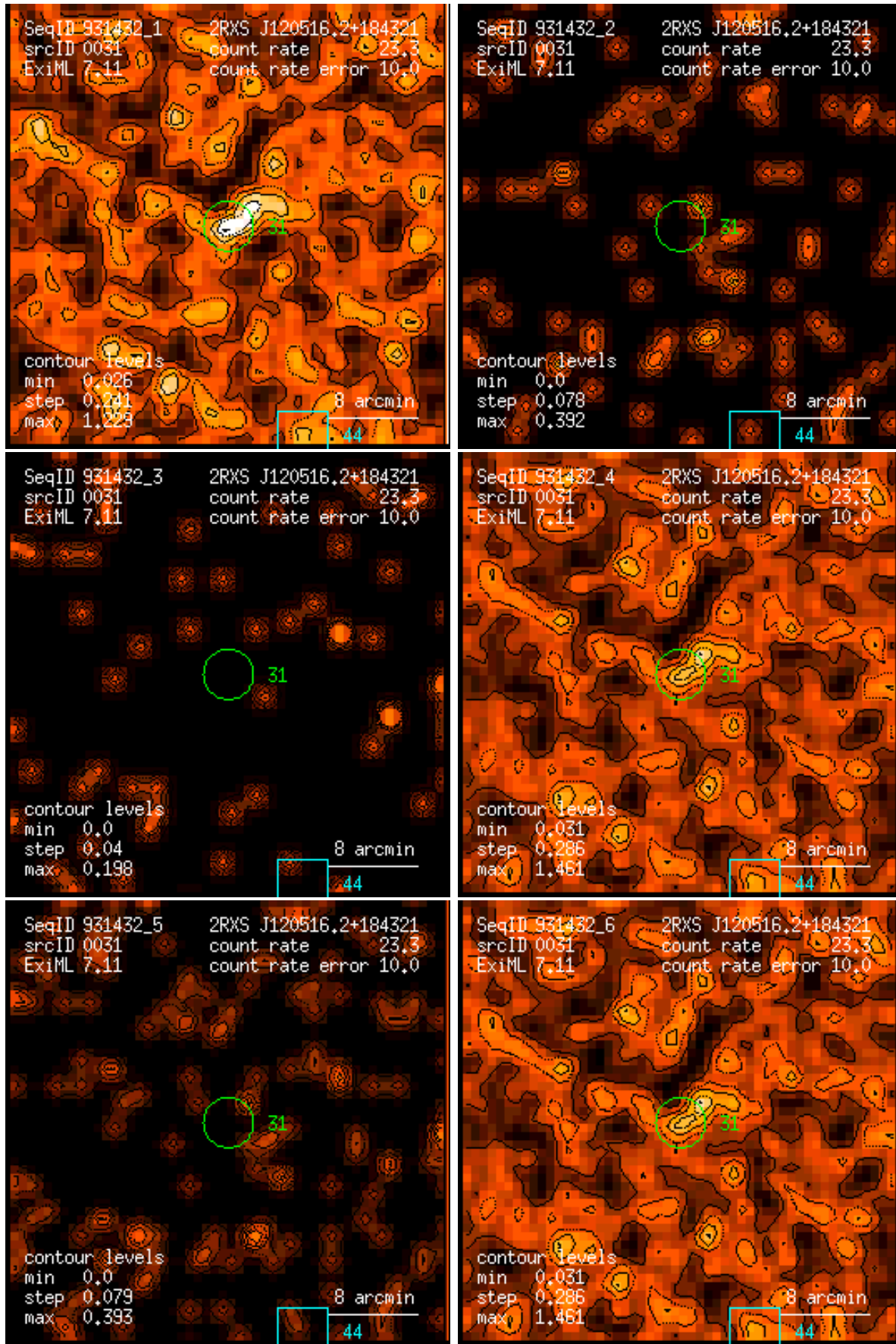
Figure 31: RASS 931432: detection 0031: band rate images, Gaussian filter: (1) PSPC channels 11 – 41, (2) 52 – 90, (3) 91 – 201, (4) 11 – 235, (5) 52 – 201, (6) 11 – 201. Broad band rates in counts/ks. Band rate contour levels in counts/ks/arcmin 2 .
