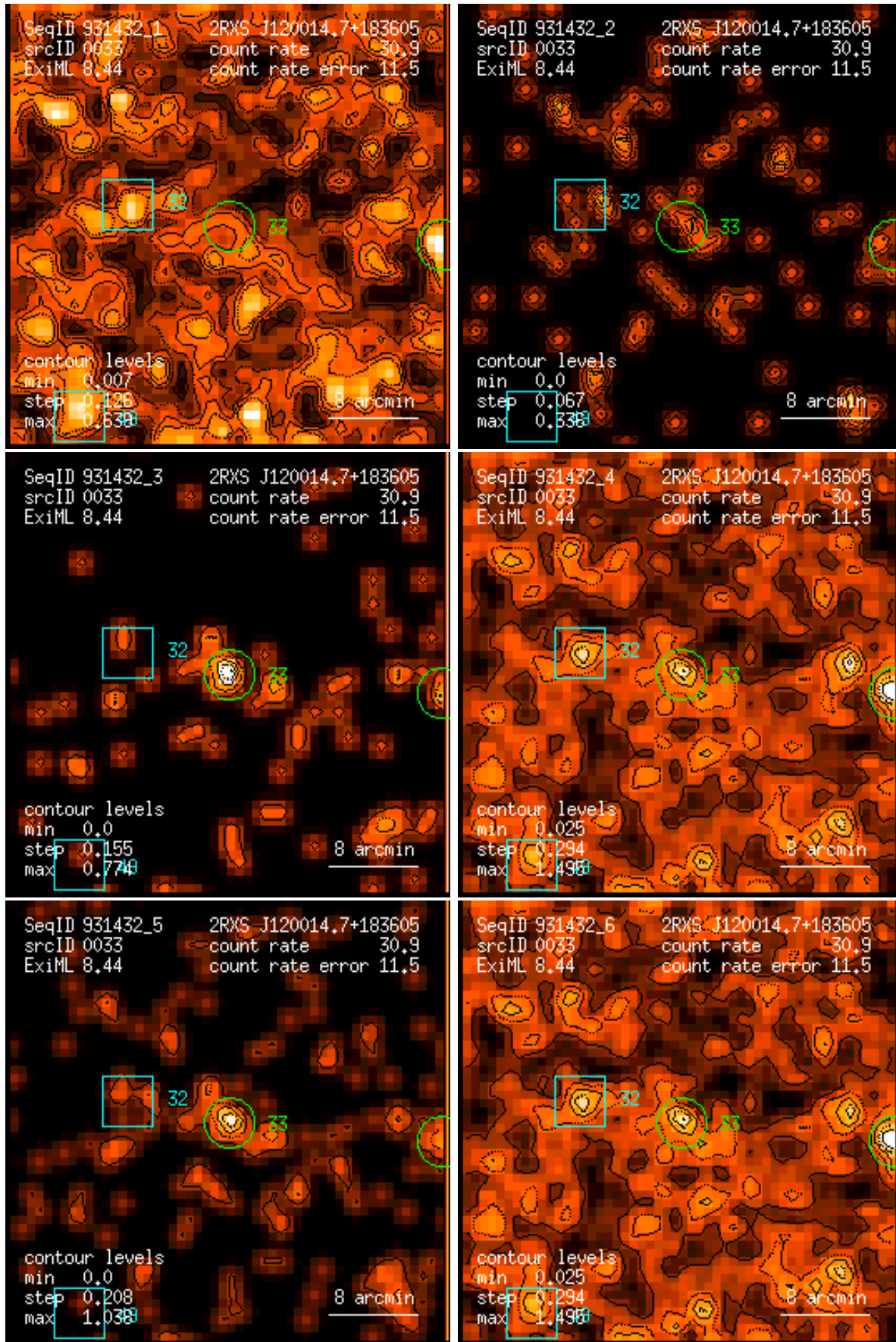
Figure 33: RASS 931432: detection 0033: band rate images, Gaussian filter: (1) PSPC channels 11 – 41, (2) 52 – 90, (3) 91 – 201, (4) 11 – 235, (5) 52 – 201, (6) 11 – 201. Broad band rates in counts/ks. Band rate contour levels in counts/ks/arcmin 2 .
