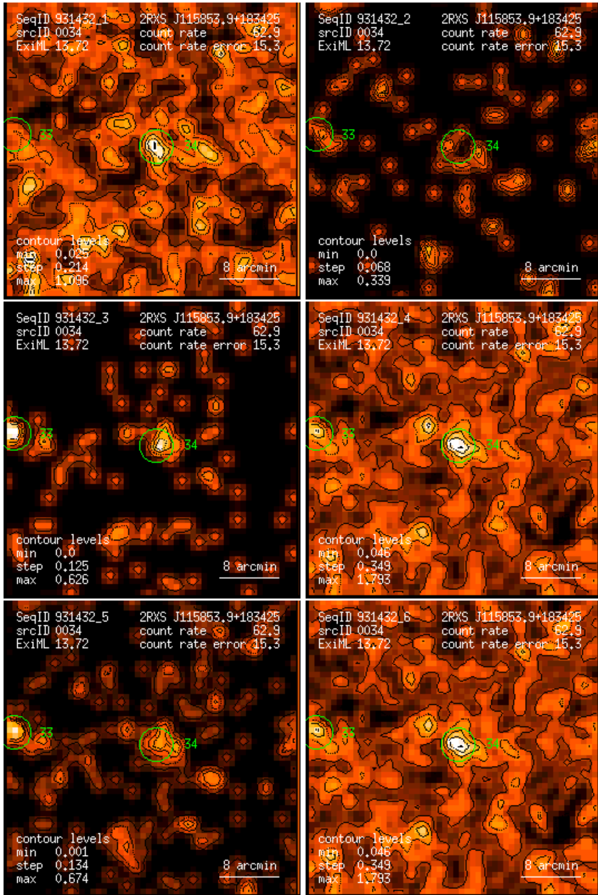
Figure 34: RASS 931432: detection 0034: band rate images, Gaussian filter: (1) PSPC channels 11 – 41, (2) 52 – 90, (3) 91 – 201, (4) 11 – 235, (5) 52 – 201, (6) 11 – 201. Broad band rates in counts/ks. Band rate contour levels in counts/ks/arcmin 2 .
