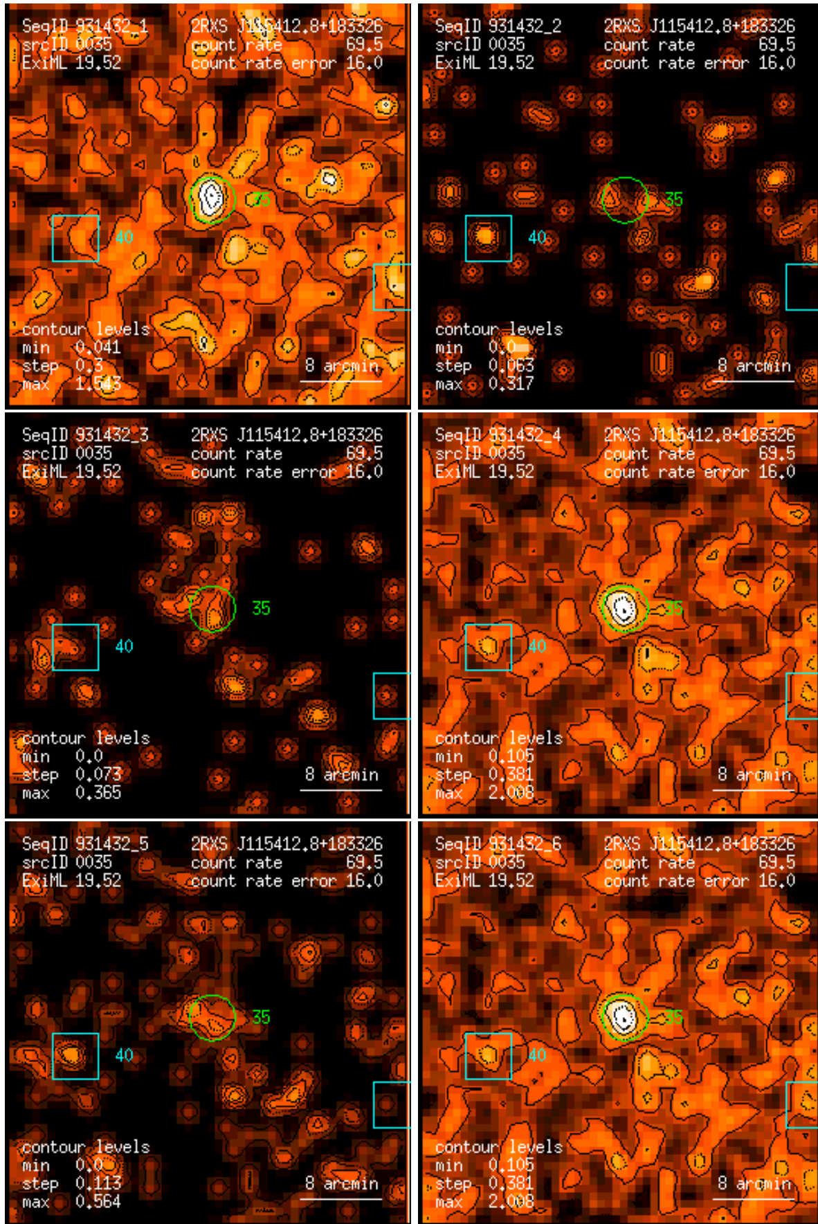
Figure 35: RASS 931432: detection 0035: band rate images, Gaussian filter: (1) PSPC channels 11 – 41, (2) 52 – 90, (3) 91 – 201, (4) 11 – 235, (5) 52 – 201, (6) 11 – 201. Broad band rates in counts/ks. Band rate contour levels in counts/ks/arcmin 2 .
