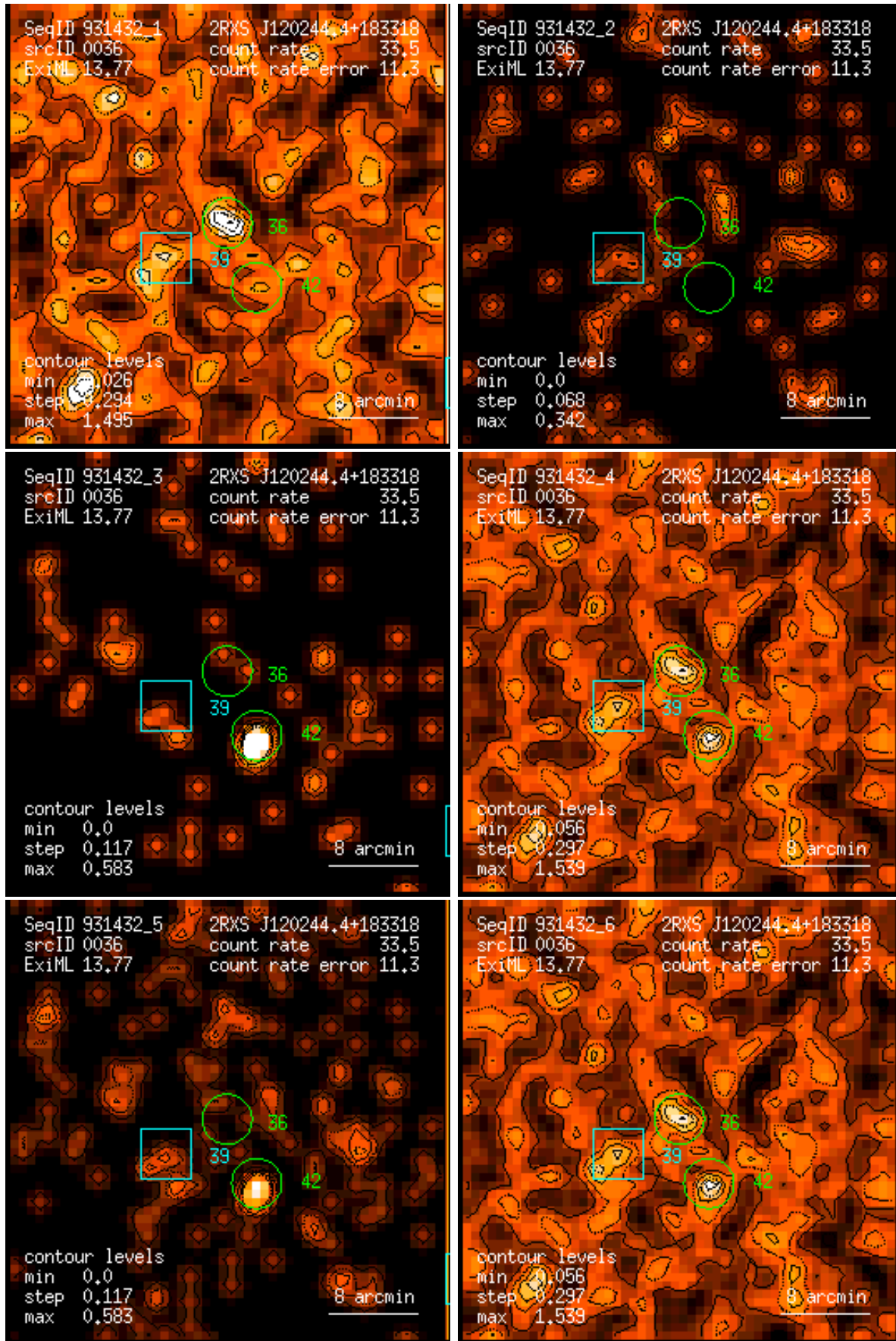
Figure 36: RASS 931432: detection 0036: band rate images, Gaussian filter: (1) PSPC channels 11 – 41, (2) 52 – 90, (3) 91 – 201, (4) 11 – 235, (5) 52 – 201, (6) 11 – 201. Broad band rates in counts/ks. Band rate contour levels in counts/ks/arcmin 2 .
