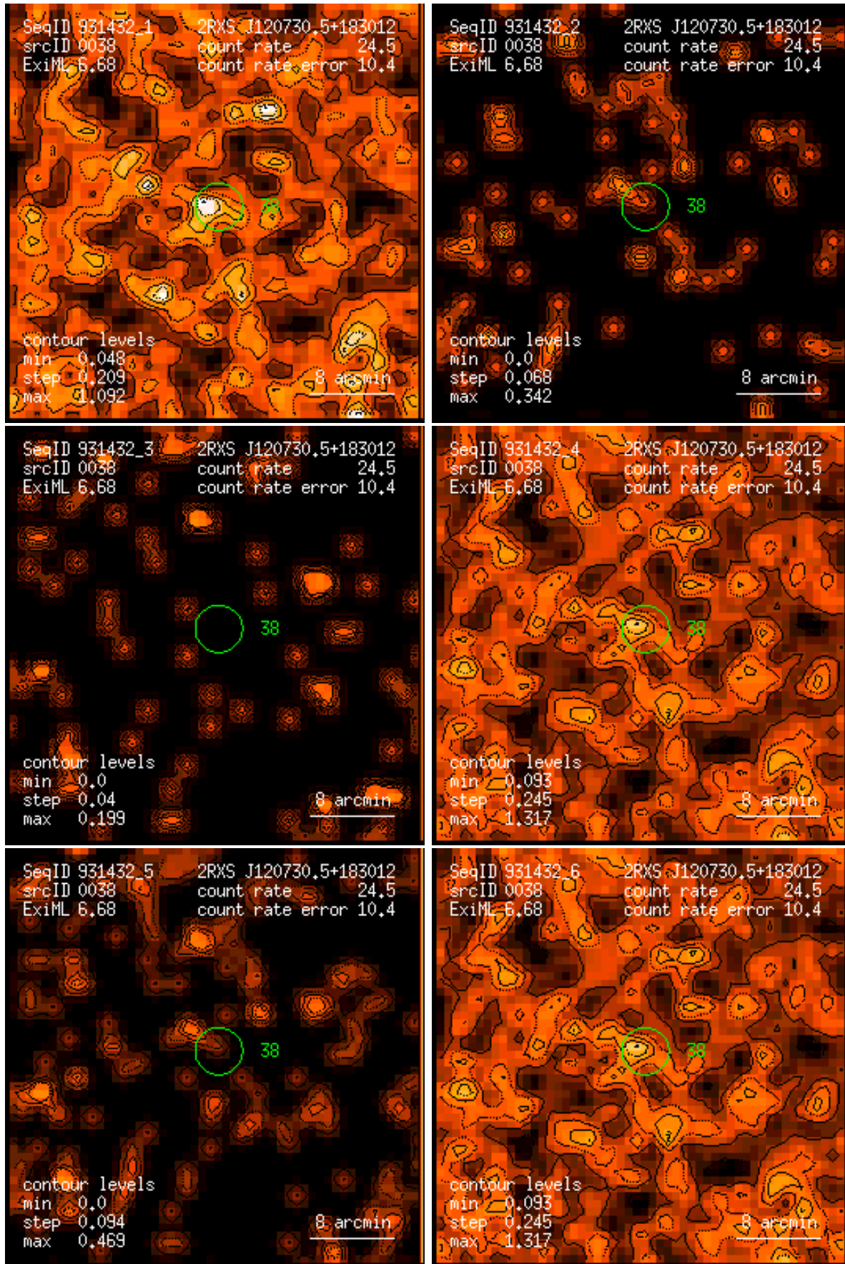
Figure 38: RASS 931432: detection 0038: band rate images, Gaussian filter: (1) PSPC channels 11 – 41, (2) 52 – 90, (3) 91 – 201, (4) 11 – 235, (5) 52 – 201, (6) 11 – 201. Broad band rates in counts/ks. Band rate contour levels in counts/ks/arcmin 2 .
