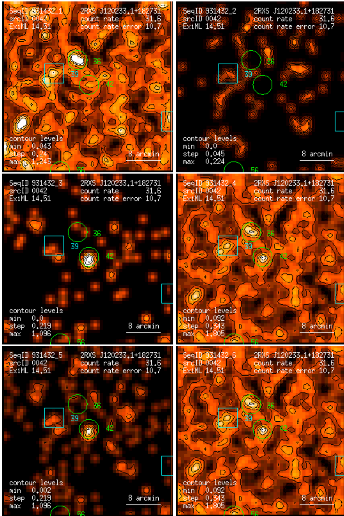
Figure 42: RASS 931432: detection 0042: band rate images, Gaussian filter: (1) PSPC channels 11 – 41, (2) 52 – 90, (3) 91 – 201, (4) 11 – 235, (5) 52 – 201, (6) 11 – 201. Broad band rates in counts/ks. Band rate contour levels in counts/ks/arcmin 2 .
