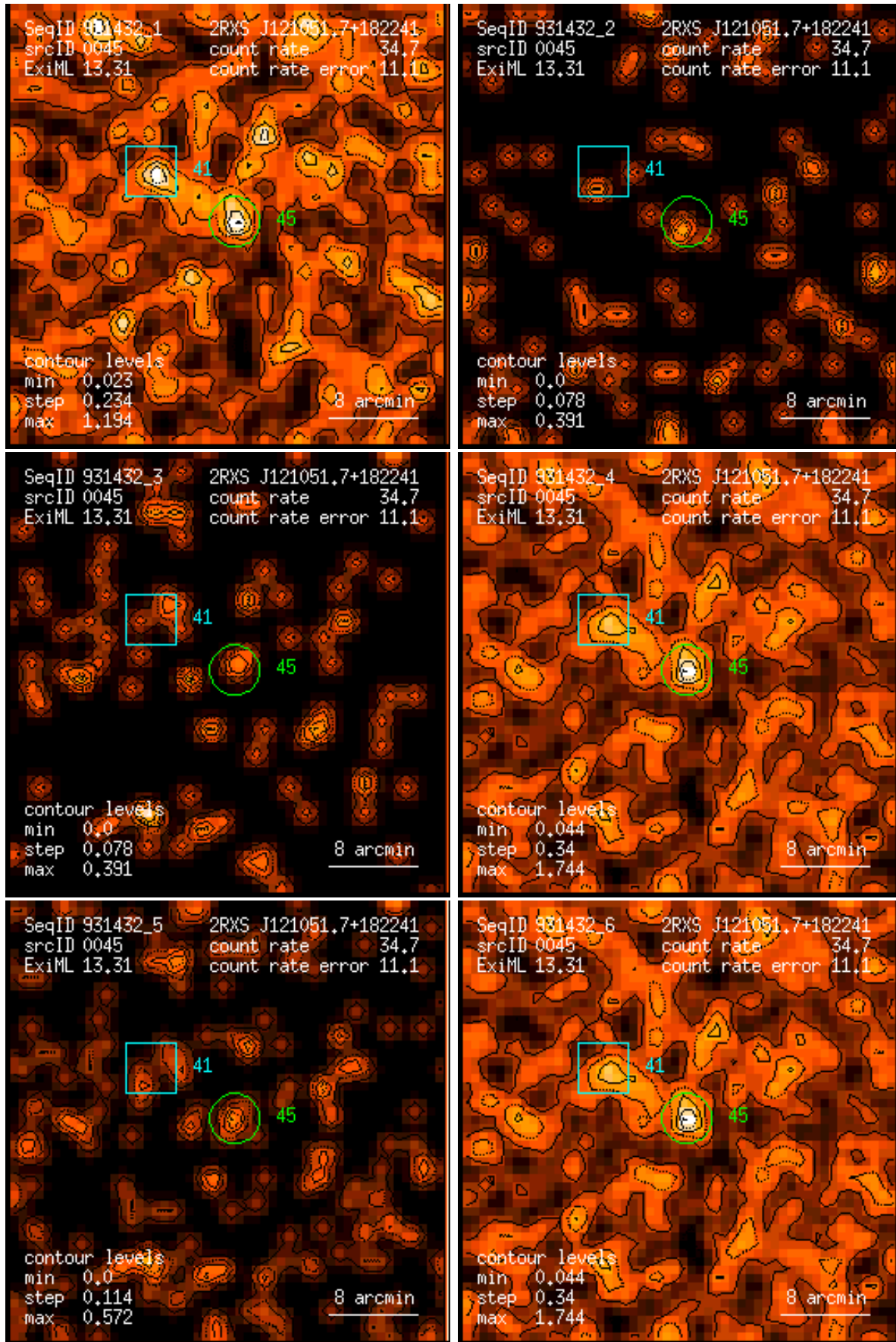
Figure 45: RASS 931432: detection 0045: band rate images, Gaussian filter: (1) PSPC channels 11 – 41, (2) 52 – 90, (3) 91 – 201, (4) 11 – 235, (5) 52 – 201, (6) 11 – 201. Broad band rates in counts/ks. Band rate contour levels in counts/ks/arcmin 2 .
