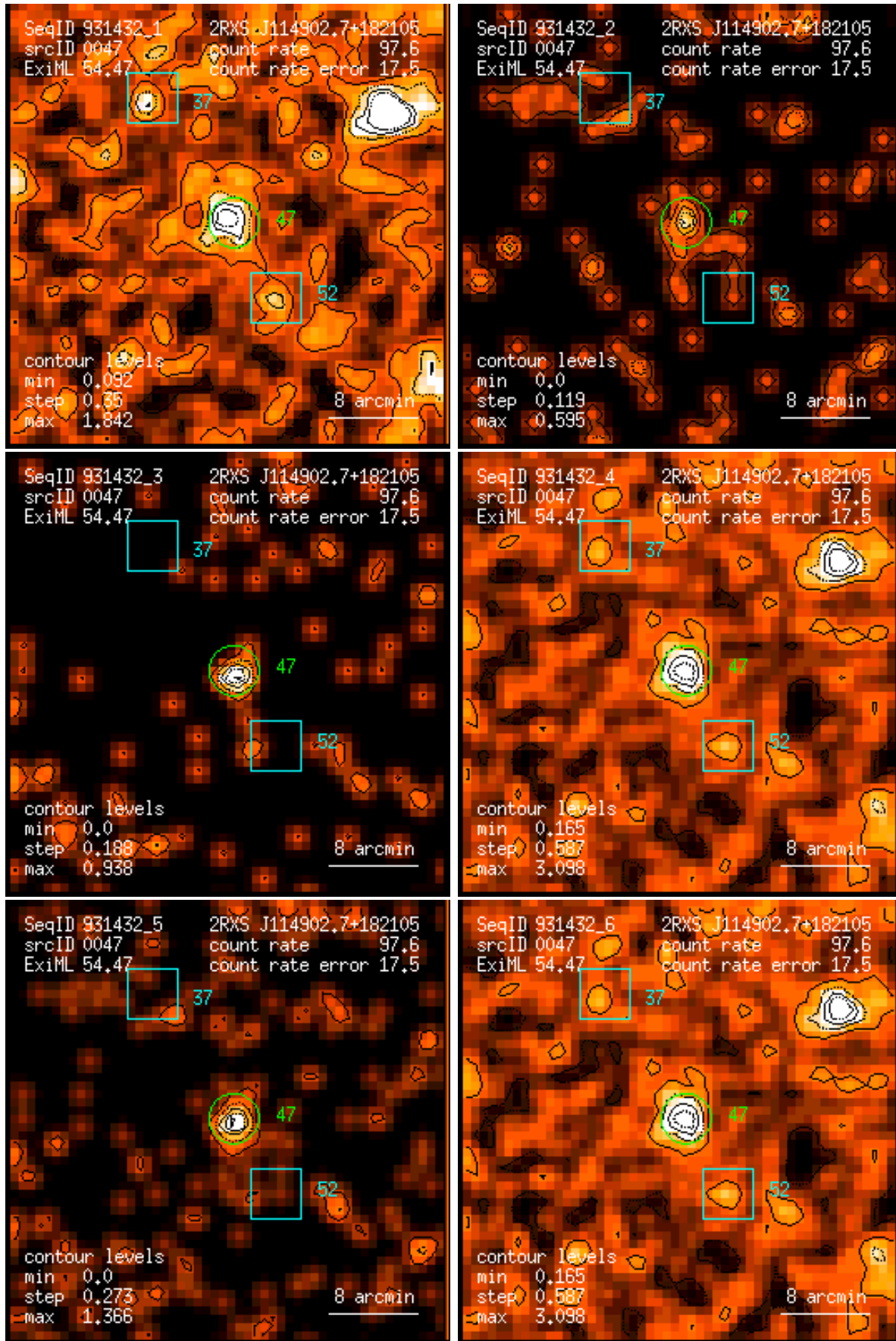
Figure 47: RASS 931432: detection 0047: band rate images, Gaussian filter: (1) PSPC channels 11 – 41, (2) 52 – 90, (3) 91 – 201, (4) 11 – 235, (5) 52 – 201, (6) 11 – 201. Broad band rates in counts/ks. Band rate contour levels in counts/ks/arcmin 2 .
