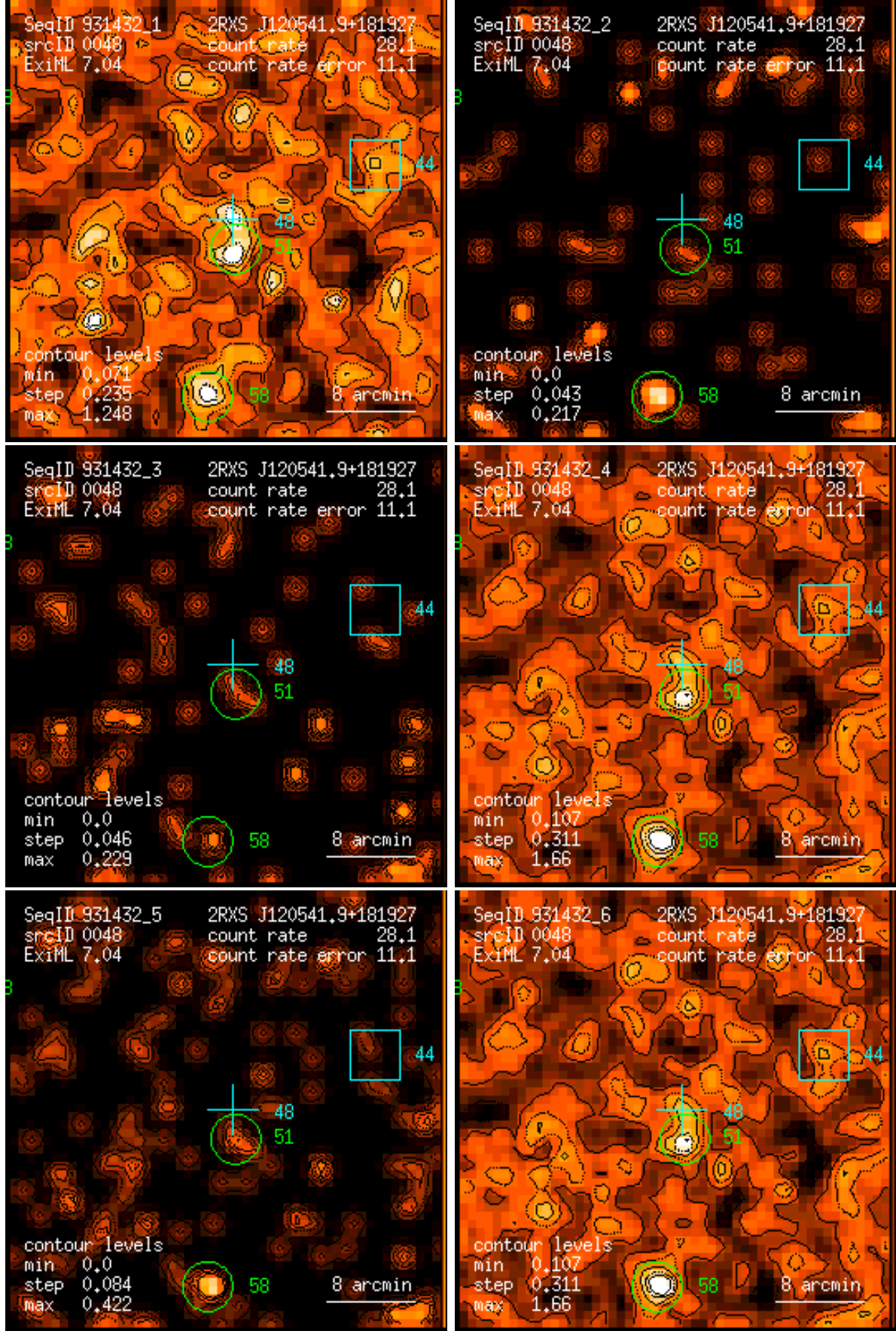
Figure 48: RASS 931432: detection 0048: band rate images, Gaussian filter: (1) PSPC channels 11 – 41, (2) 52 – 90, (3) 91 – 201, (4) 11 – 235, (5) 52 – 201, (6) 11 – 201. Broad band rates in counts/ks. Band rate contour levels in counts/ks/arcmin 2 .
