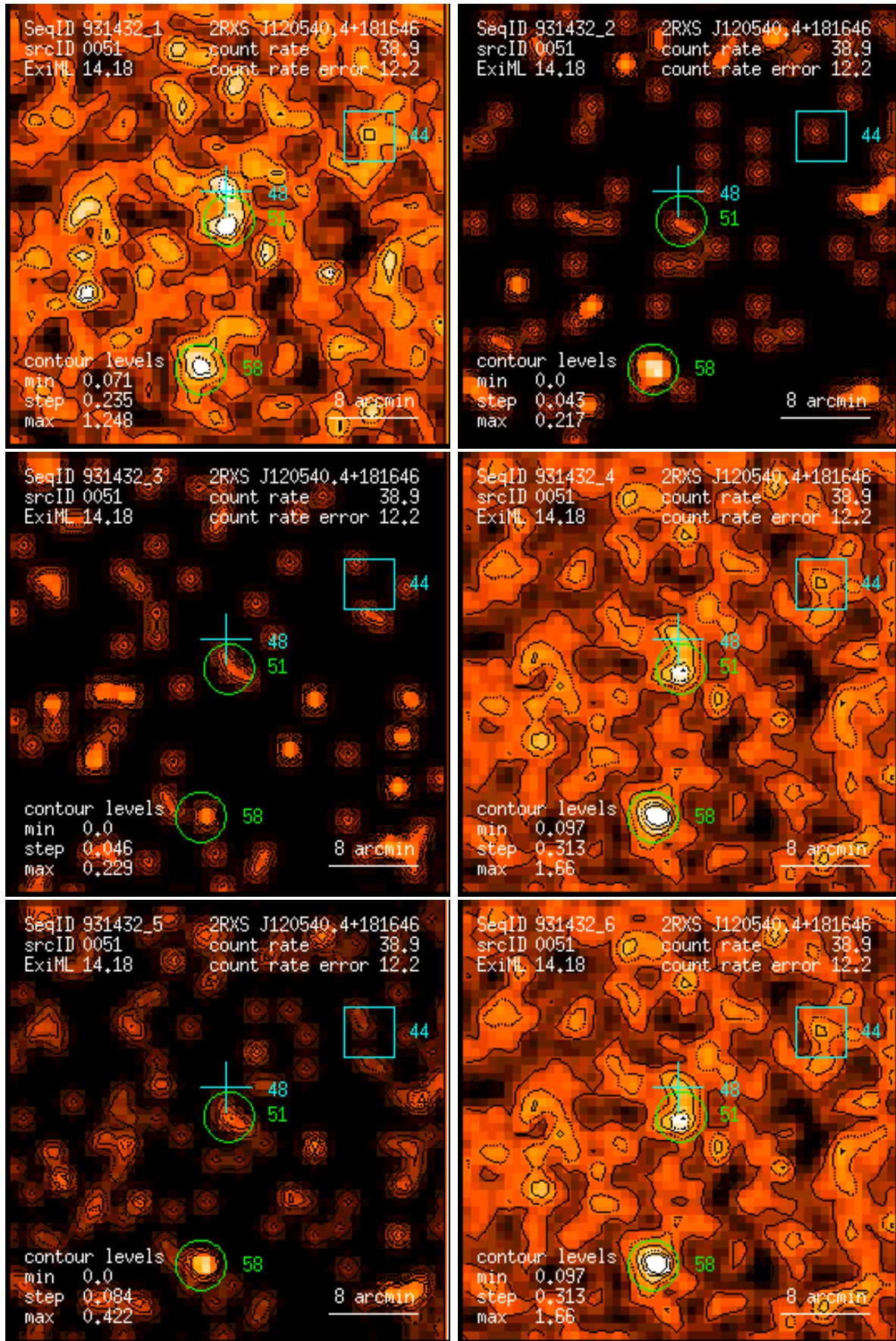
Figure 51: RASS 931432: detection 0051: band rate images, Gaussian filter: (1) PSPC channels 11 – 41, (2) 52 – 90, (3) 91 – 201, (4) 11 – 235, (5) 52 – 201, (6) 11 – 201. Broad band rates in counts/ks. Band rate contour levels in counts/ks/arcmin 2 .
