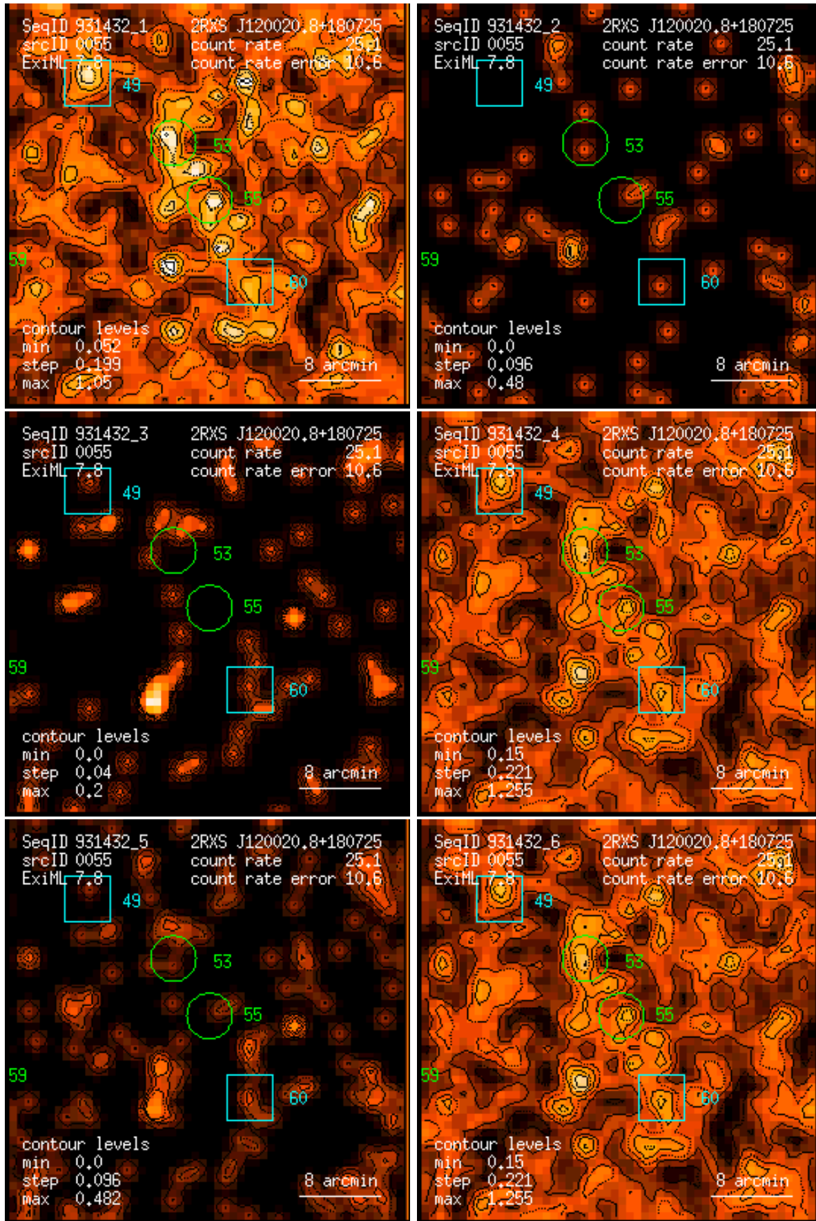
Figure 55: RASS 931432: detection 0055: band rate images, Gaussian filter: (1) PSPC channels 11 – 41, (2) 52 – 90, (3) 91 – 201, (4) 11 – 235, (5) 52 – 201, (6) 11 – 201. Broad band rates in counts/ks. Band rate contour levels in counts/ks/arcmin 2 .
