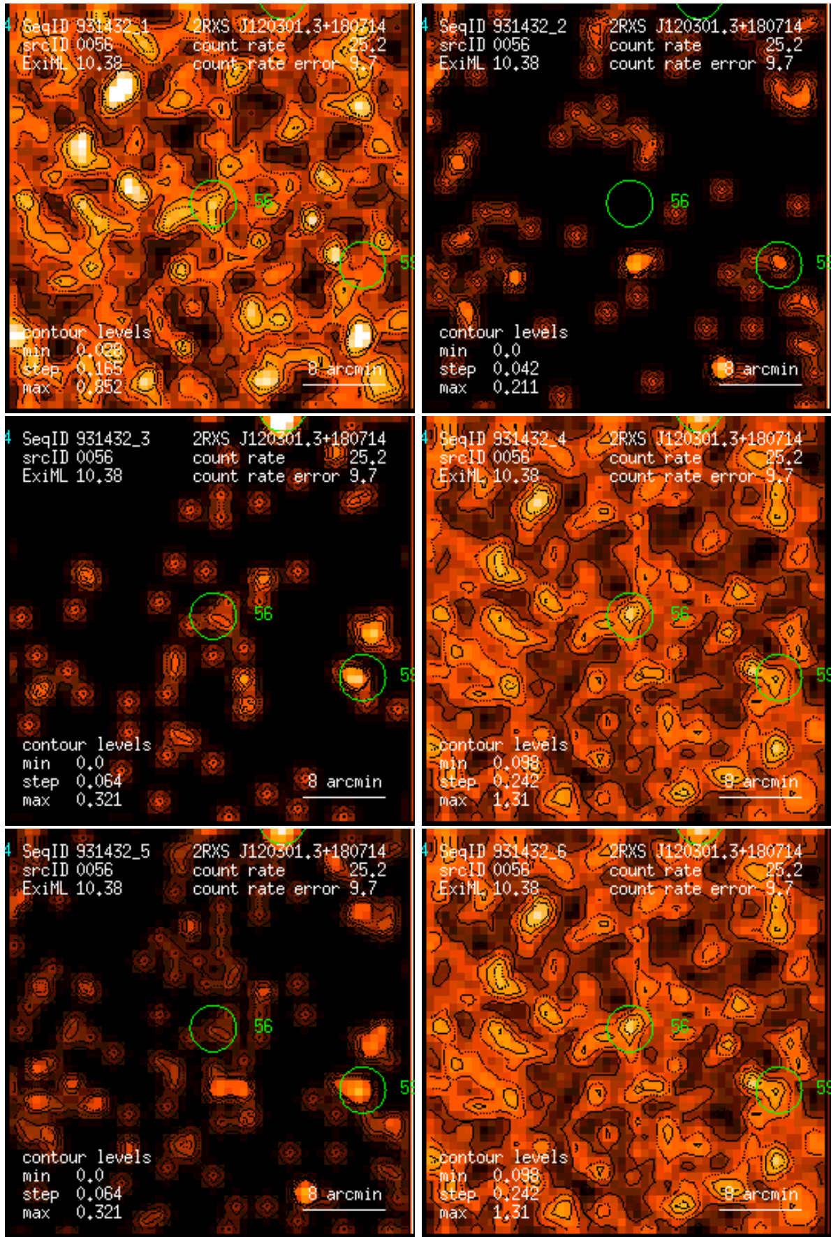
Figure 56: RASS 931432: detection 0056: band rate images, Gaussian filter: (1) PSPC channels 11 – 41, (2) 52 – 90, (3) 91 – 201, (4) 11 – 235, (5) 52 – 201, (6) 11 – 201. Broad band rates in counts/ks. Band rate contour levels in counts/ks/arcmin 2 .
