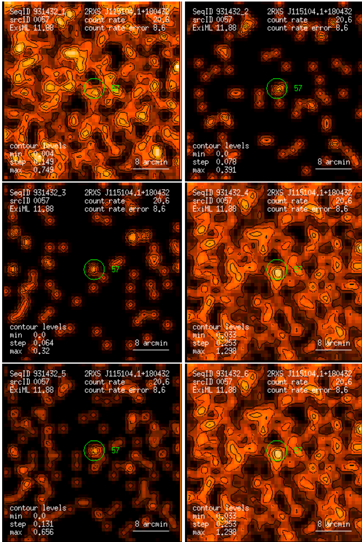
Figure 57: RASS 931432: detection 0057: band rate images, Gaussian filter: (1) PSPC channels 11 – 41, (2) 52 – 90, (3) 91 – 201, (4) 11 – 235, (5) 52 – 201, (6) 11 – 201. Broad band rates in counts/ks. Band rate contour levels in counts/ks/arcmin 2 .
