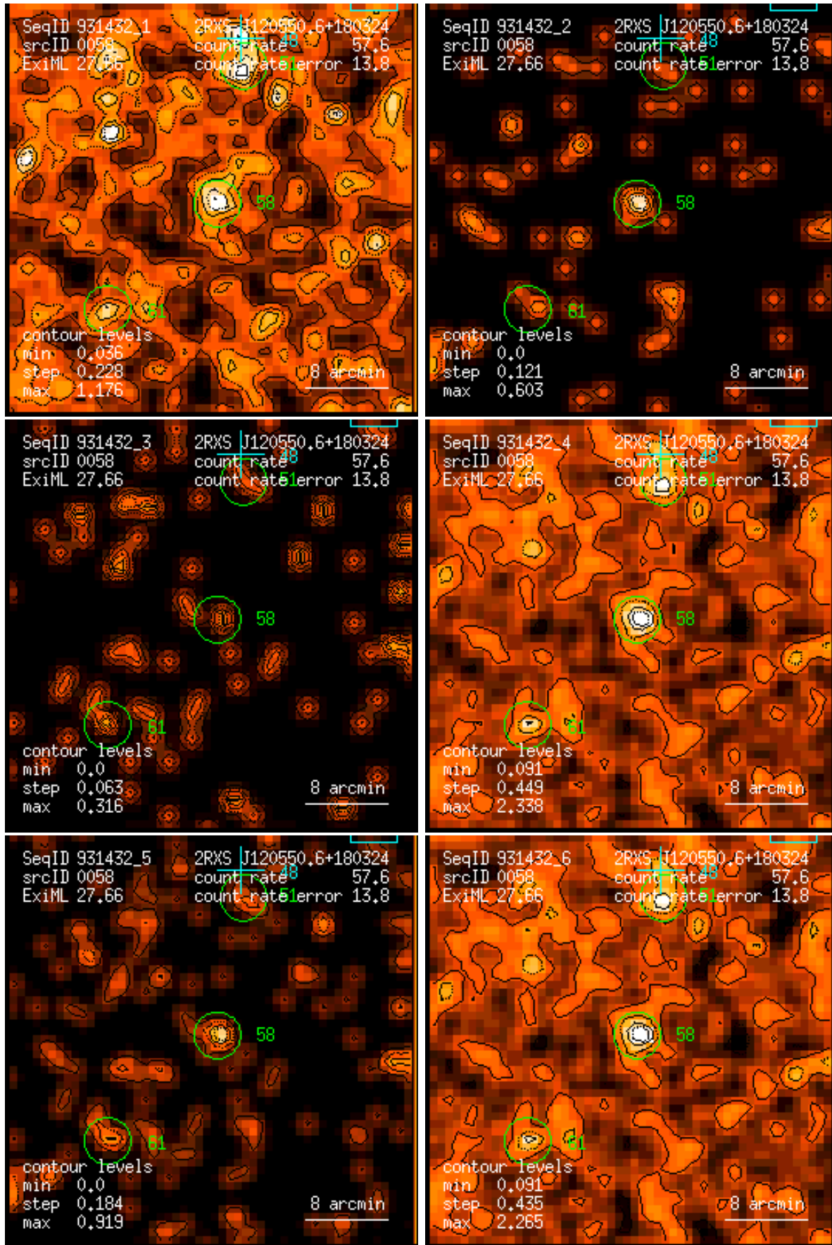
Figure 58: RASS 931432: detection 0058: band rate images, Gaussian filter: (1) PSPC channels 11 – 41, (2) 52 – 90, (3) 91 – 201, (4) 11 – 235, (5) 52 – 201, (6) 11 – 201. Broad band rates in counts/ks. Band rate contour levels in counts/ks/arcmin 2 .
