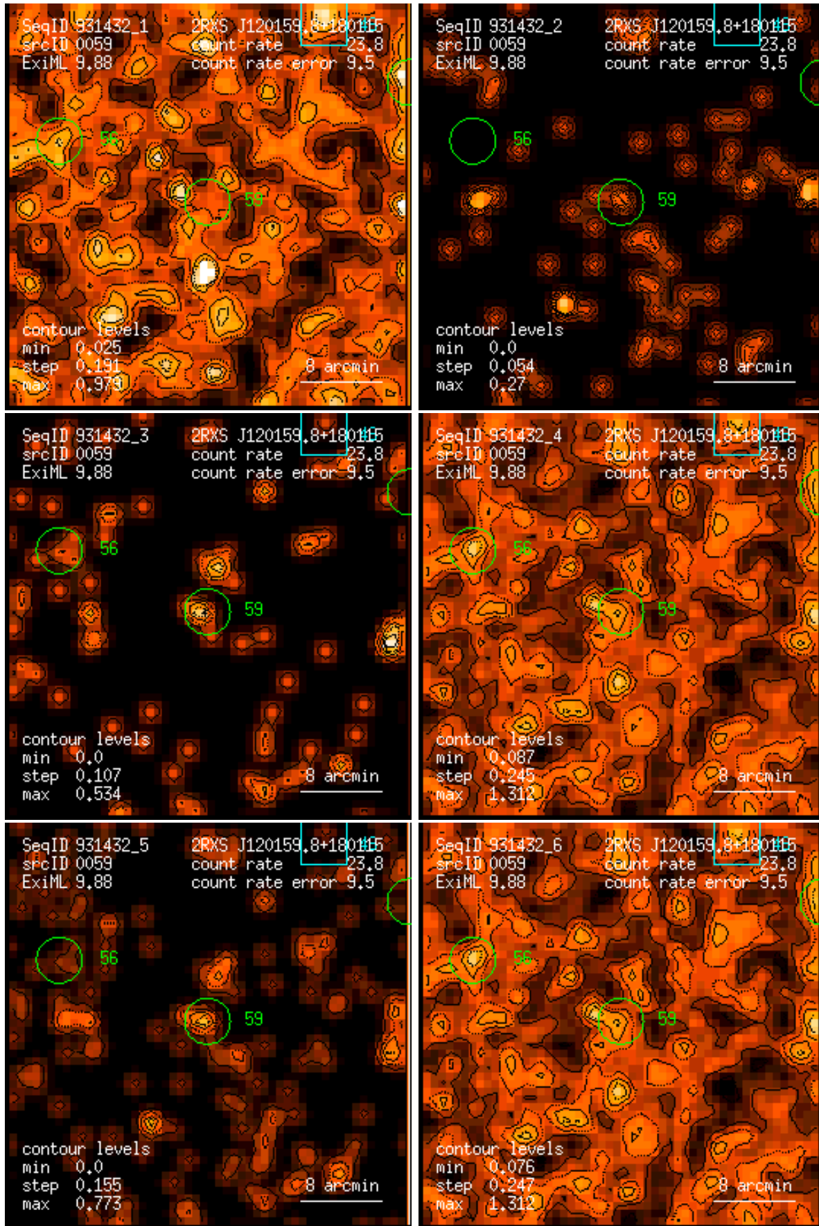
Figure 59: RASS 931432: detection 0059: band rate images, Gaussian filter: (1) PSPC channels 11 – 41, (2) 52 – 90, (3) 91 – 201, (4) 11 – 235, (5) 52 – 201, (6) 11 – 201. Broad band rates in counts/ks. Band rate contour levels in counts/ks/arcmin 2 .
