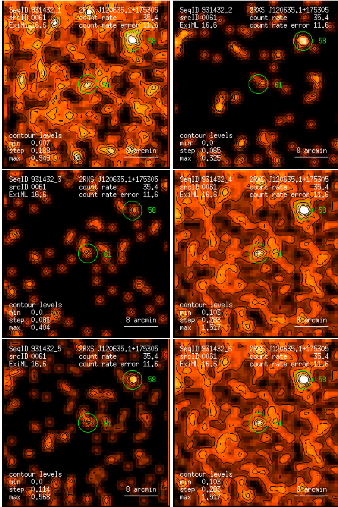
Figure 61: RASS 931432: detection 0061: band rate images, Gaussian filter: (1) PSPC channels 11 – 41, (2) 52 – 90, (3) 91 – 201, (4) 11 – 235, (5) 52 – 201, (6) 11 – 201. Broad band rates in counts/ks. Band rate contour levels in counts/ks/arcmin 2 .
