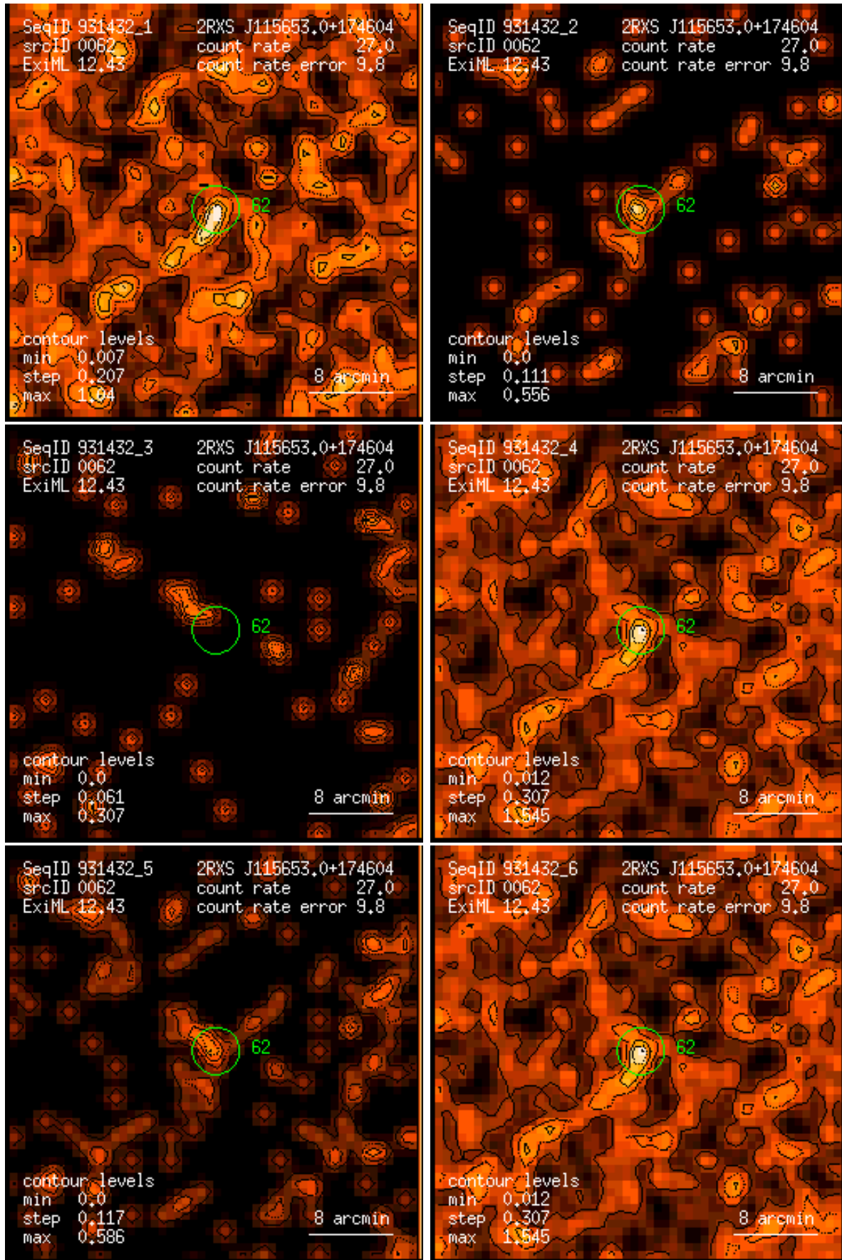
Figure 62: RASS 931432: detection 0062: band rate images, Gaussian filter: (1) PSPC channels 11 – 41, (2) 52 – 90, (3) 91 – 201, (4) 11 – 235, (5) 52 – 201, (6) 11 – 201. Broad band rates in counts/ks. Band rate contour levels in counts/ks/arcmin 2 .
