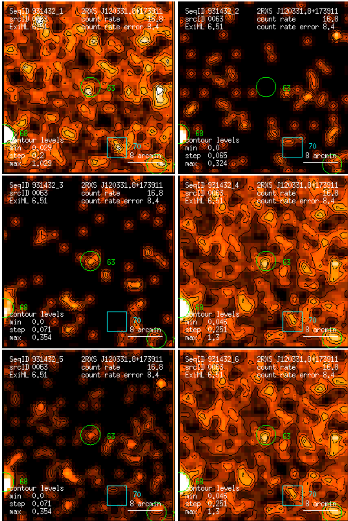
Figure 63: RASS 931432: detection 0063: band rate images, Gaussian filter: (1) PSPC channels 11 – 41, (2) 52 – 90, (3) 91 – 201, (4) 11 – 235, (5) 52 – 201, (6) 11 – 201. Broad band rates in counts/ks. Band rate contour levels in counts/ks/arcmin 2 .
