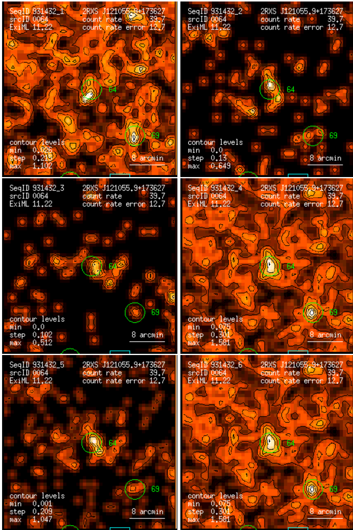
Figure 64: RASS 931432: detection 0064: band rate images, Gaussian filter: (1) PSPC channels 11 – 41, (2) 52 – 90, (3) 91 – 201, (4) 11 – 235, (5) 52 – 201, (6) 11 – 201. Broad band rates in counts/ks. Band rate contour levels in counts/ks/arcmin 2 .
