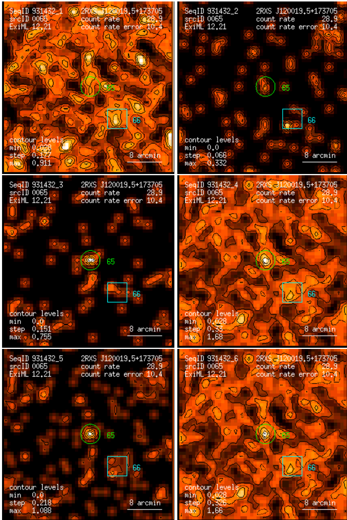
Figure 65: RASS 931432: detection 0065: band rate images, Gaussian filter: (1) PSPC channels 11 – 41, (2) 52 – 90, (3) 91 – 201, (4) 11 – 235, (5) 52 – 201, (6) 11 – 201. Broad band rates in counts/ks. Band rate contour levels in counts/ks/arcmin 2 .
