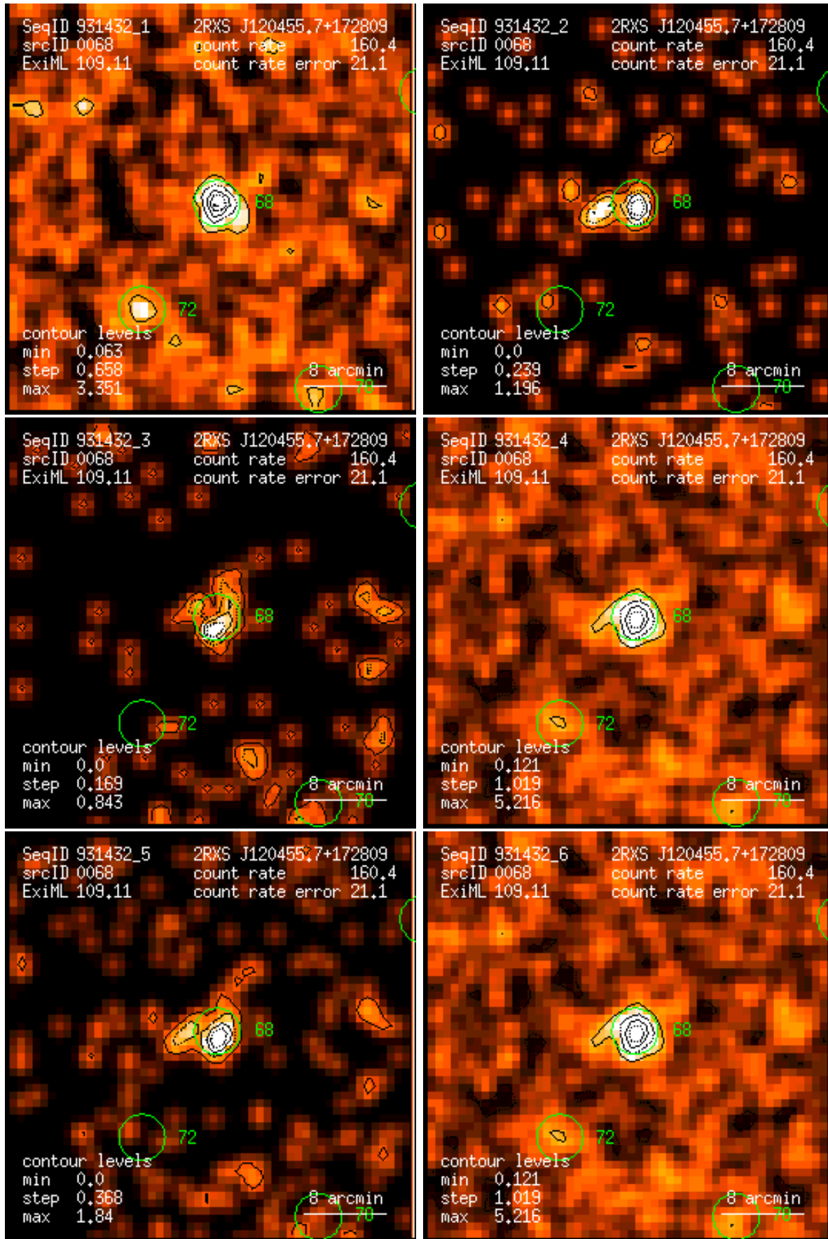
Figure 68: RASS 931432: detection 0068: band rate images, Gaussian filter: (1) PSPC channels 11 – 41, (2) 52 – 90, (3) 91 – 201, (4) 11 – 235, (5) 52 – 201, (6) 11 – 201. Broad band rates in counts/ks. Band rate contour levels in counts/ks/arcmin 2 .
