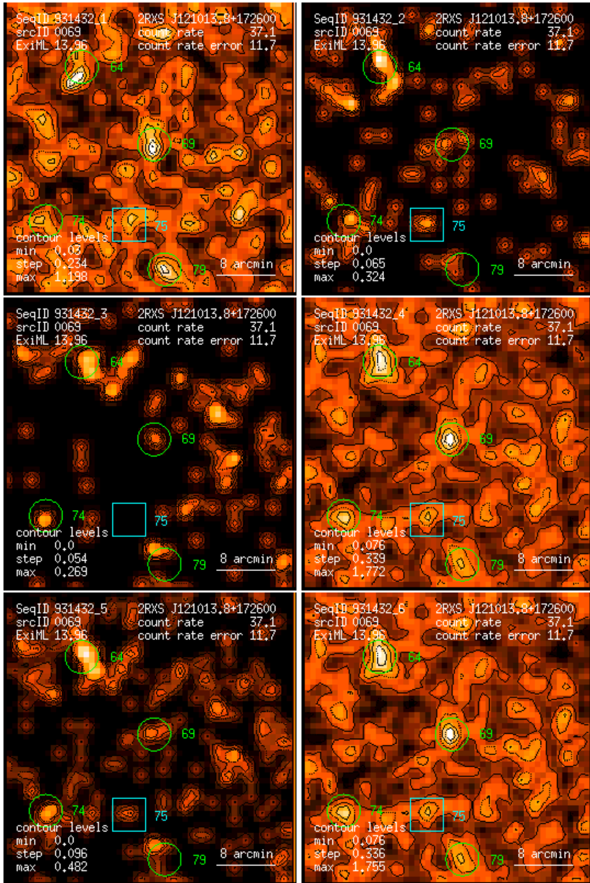
Figure 69: RASS 931432: detection 0069: band rate images, Gaussian filter: (1) PSPC channels 11 – 41, (2) 52 – 90, (3) 91 – 201, (4) 11 – 235, (5) 52 – 201, (6) 11 – 201. Broad band rates in counts/ks. Band rate contour levels in counts/ks/arcmin 2 .
