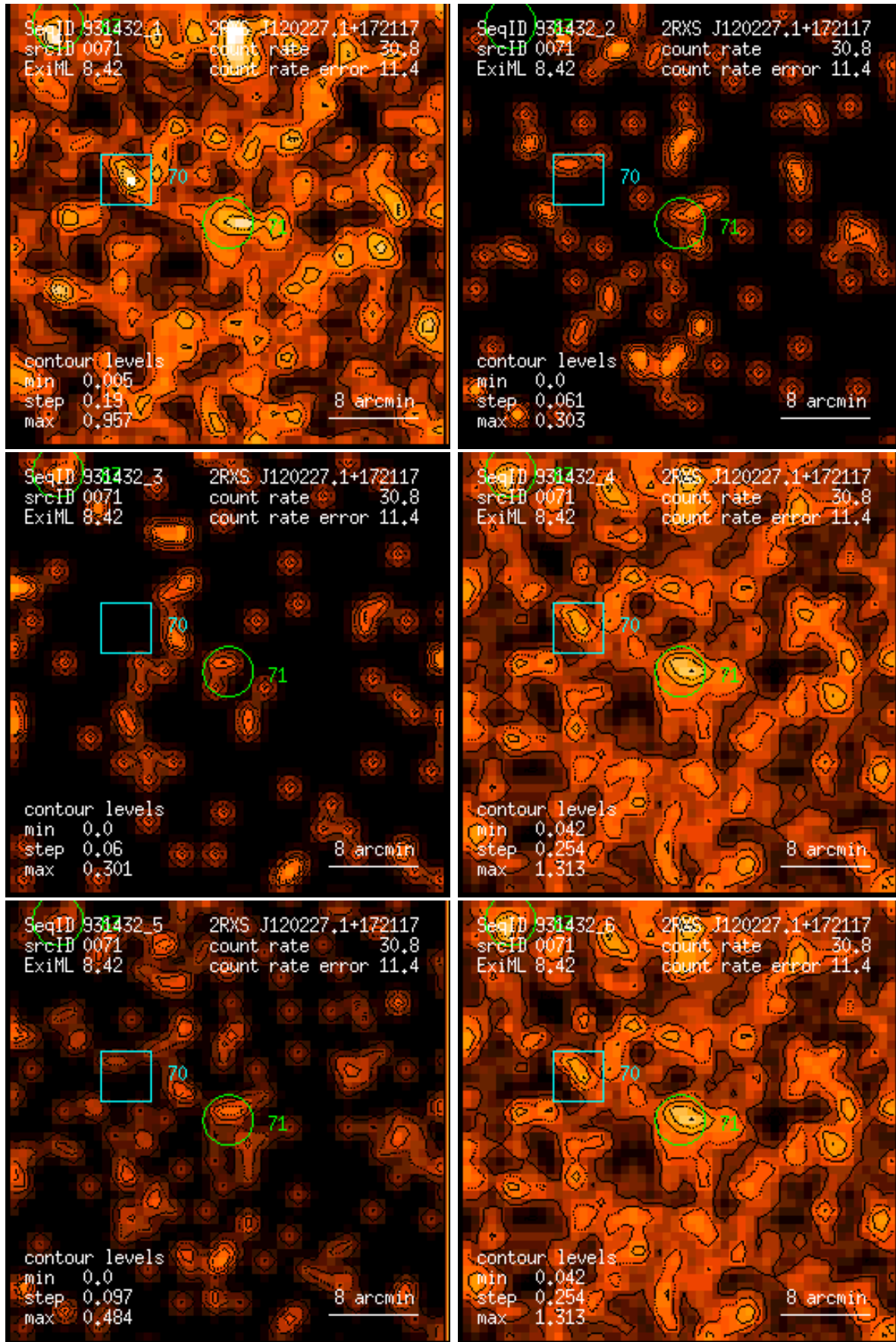
Figure 71: RASS 931432: detection 0071: band rate images, Gaussian filter: (1) PSPC channels 11 – 41, (2) 52 – 90, (3) 91 – 201, (4) 11 – 235, (5) 52 – 201, (6) 11 – 201. Broad band rates in counts/ks. Band rate contour levels in counts/ks/arcmin 2 .
