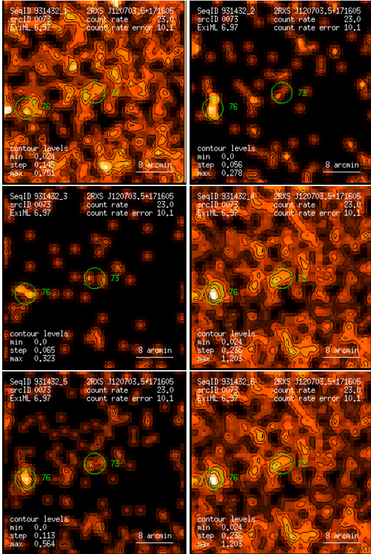
Figure 73: RASS 931432: detection 0073: band rate images, Gaussian filter: (1) PSPC channels 11 – 41, (2) 52 – 90, (3) 91 – 201, (4) 11 – 235, (5) 52 – 201, (6) 11 – 201. Broad band rates in counts/ks. Band rate contour levels in counts/ks/arcmin 2 .
